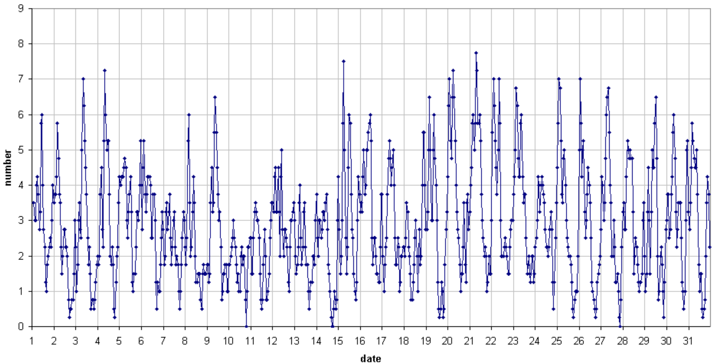
49.99MHz - RadioMeteors October 2017 number of overdense reflections per hour (weighted average) Felix Verbelen (Kamphenhout)
