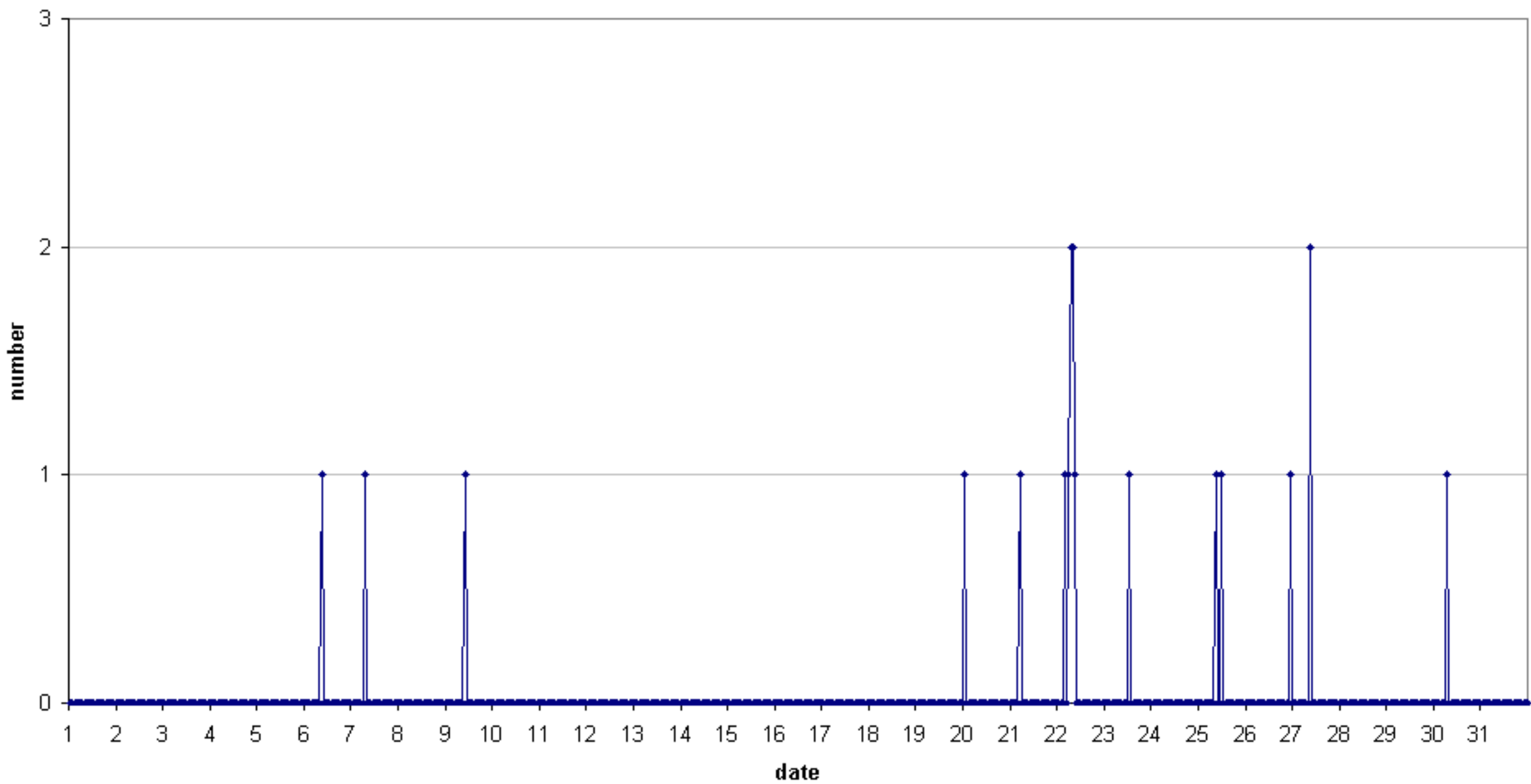
49.99MHz - RadioMeteors October 2017 hourly totals of overdense reflections longer than 1 minute Felix Verbelen (Kamphenhout/BE)
