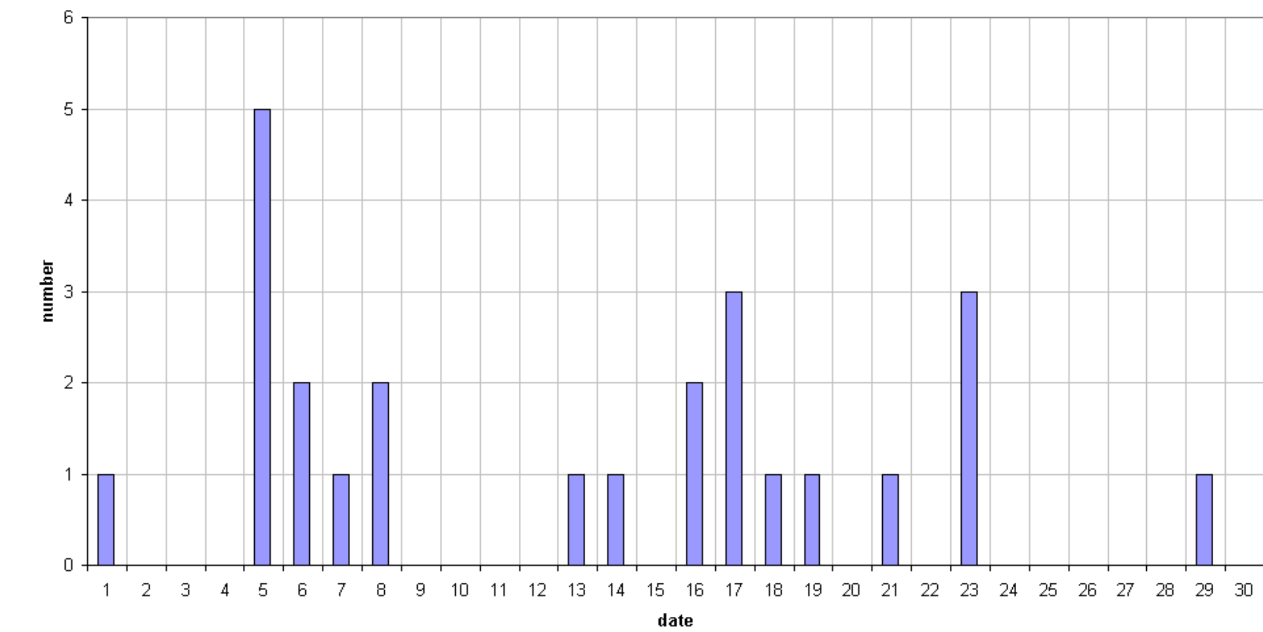
49.99MHz - RadioMeteors November 2017 daily totals of reflections longer than 1 minute Felix Verbelen (Kampenhout)
