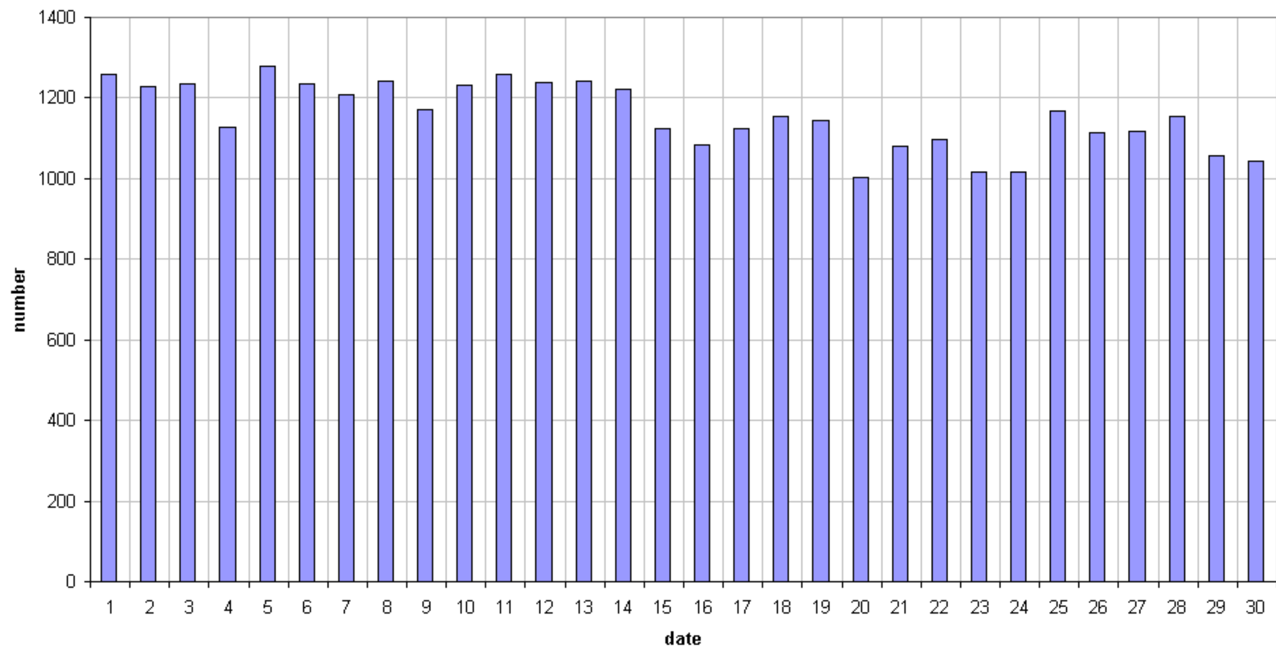
49.99MHz - RadioMeteors November 2017 daily totals of "all" reflections (automatic count_Mettel5_7Hz) Felix Verbelen (Kampenhout)
