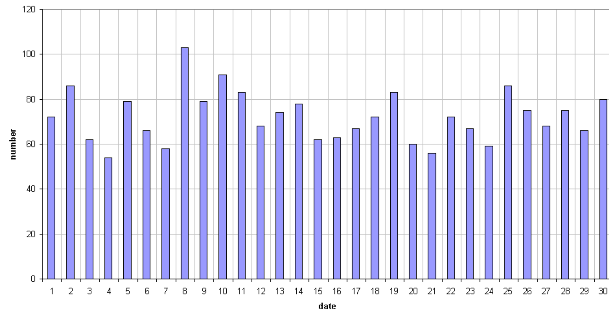
49.99MHz - RadioMeteors November 2017 daily totals of all overdense reflections Felix Verbelen (Kampenhout)
