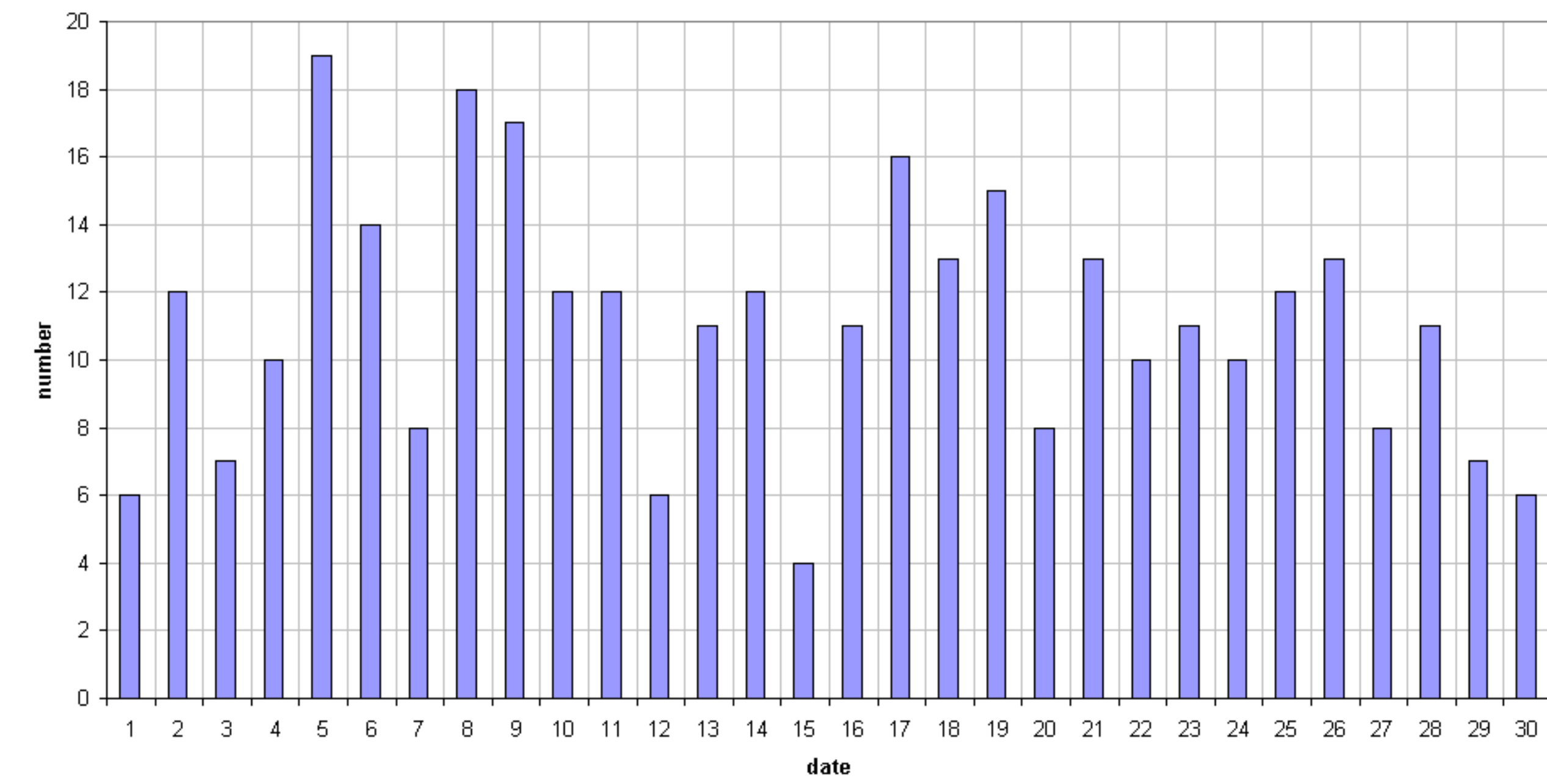
49.99MHz - RadioMeteors November 2017 daily totals of reflections longer than 10 seconds Felix Verbelen (Kampenhout)
