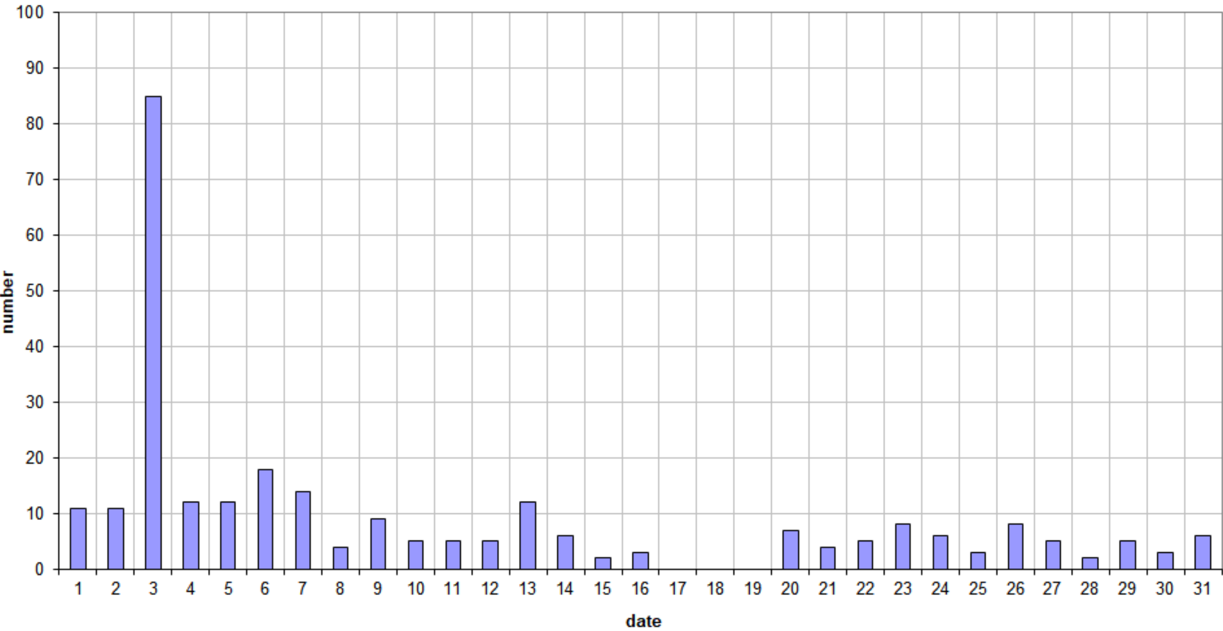
49.99MHz - RadioMeteors January 2025 daily totals of reflections longer than 10 seconds Felix Verbelen (Kampenhout)
