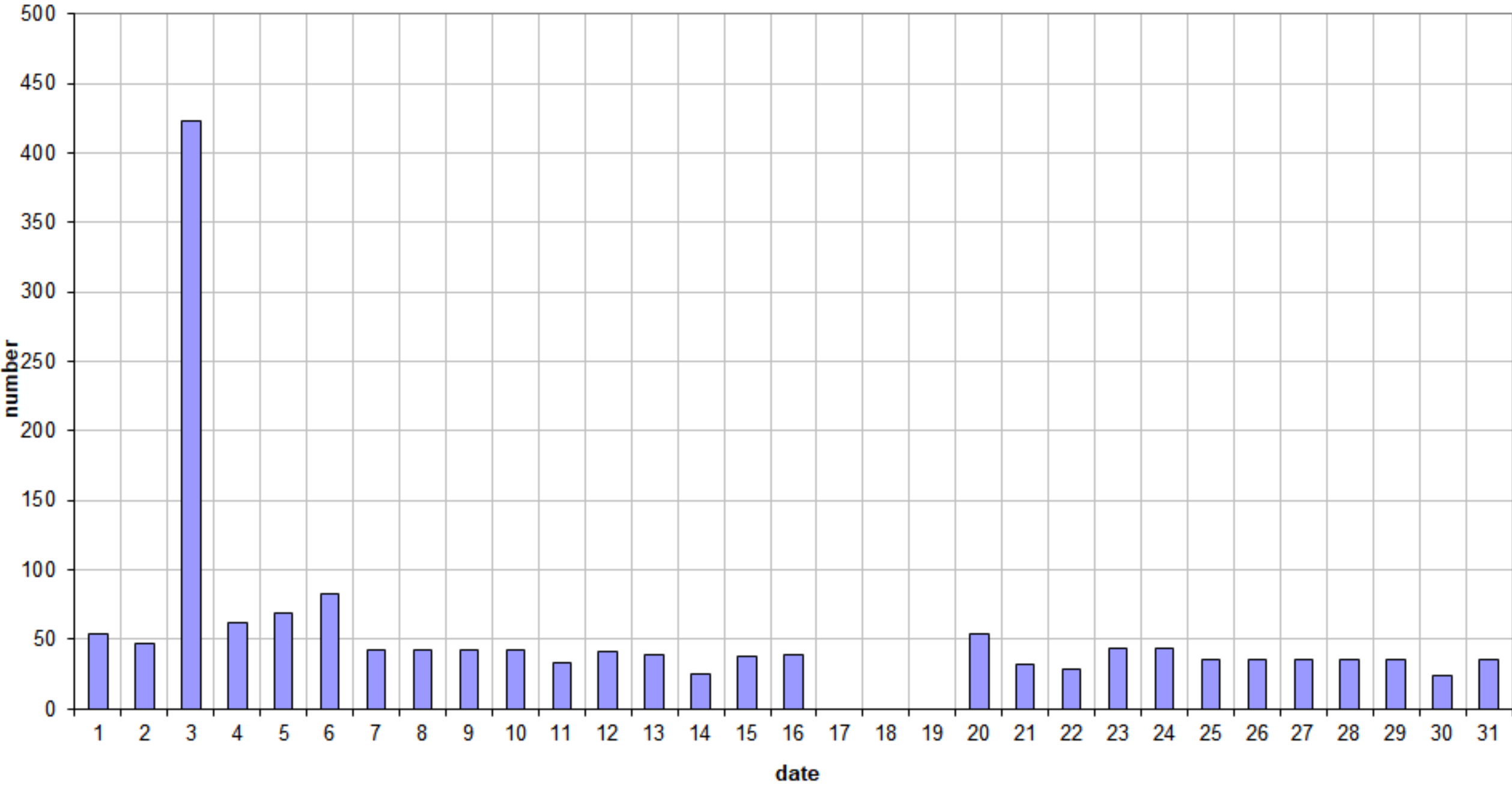
49.99MHz - RadioMeteors January 2025 daily totals of all overdense reflections Felix Verbelen (Kampenhout)
