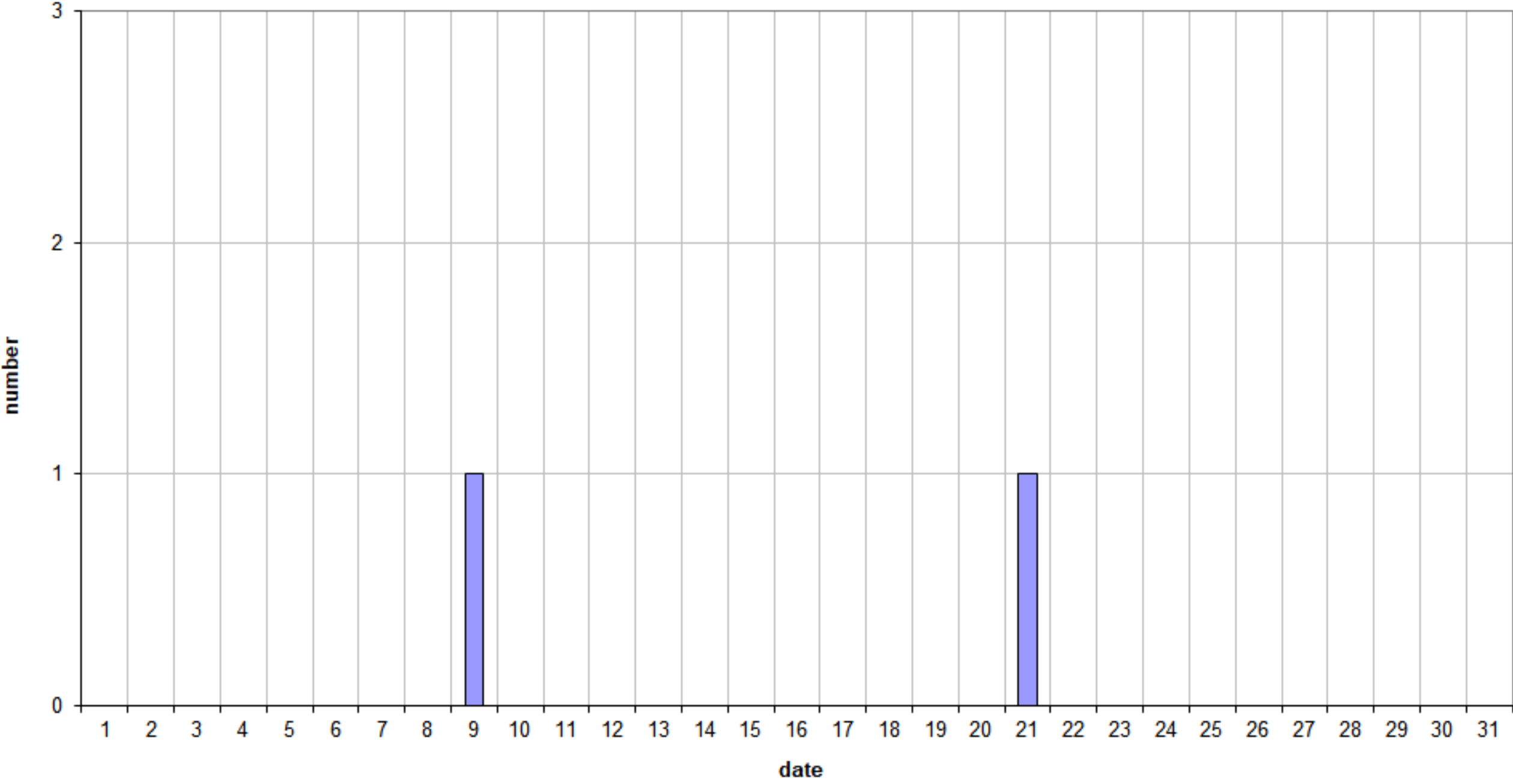
49.99MHz - RadioMeteors January 2025 daily totals of reflections longer than 1 minute Felix Verbelen (Kampenhout)
