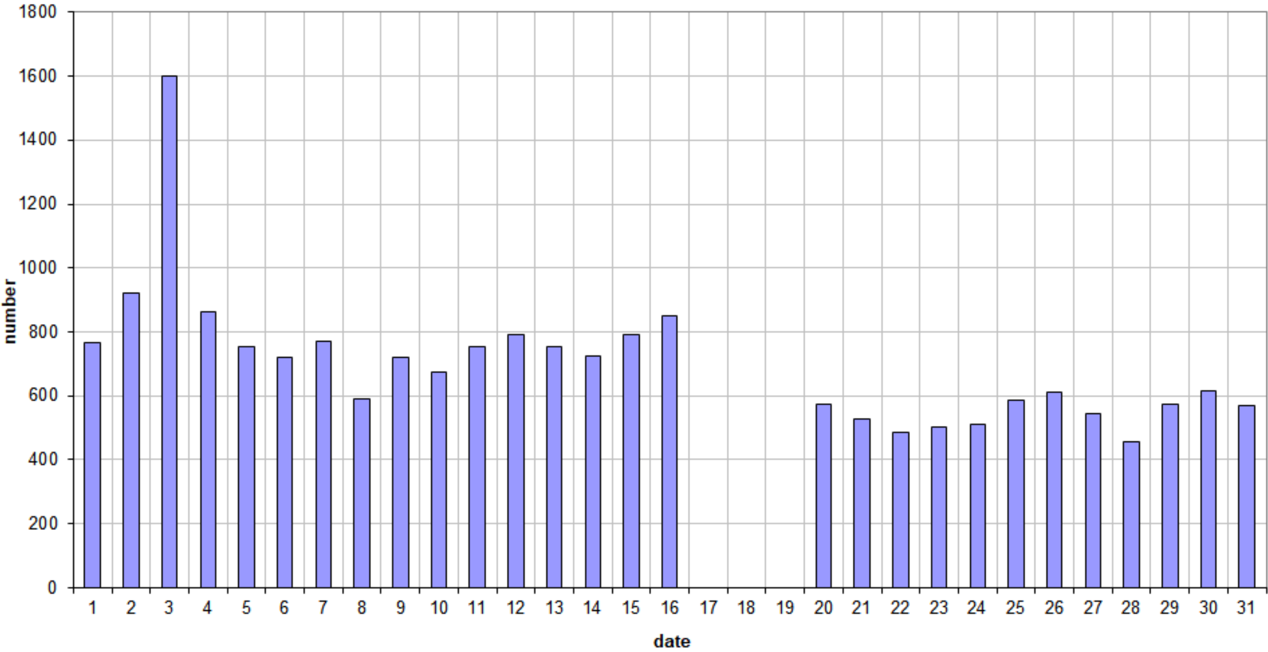
49.99MHz - RadioMeteors January 2025 daily totals of "all" reflections (automatic count_Mettel5_7Hz) Felix Verbelen (Kampenhout)
