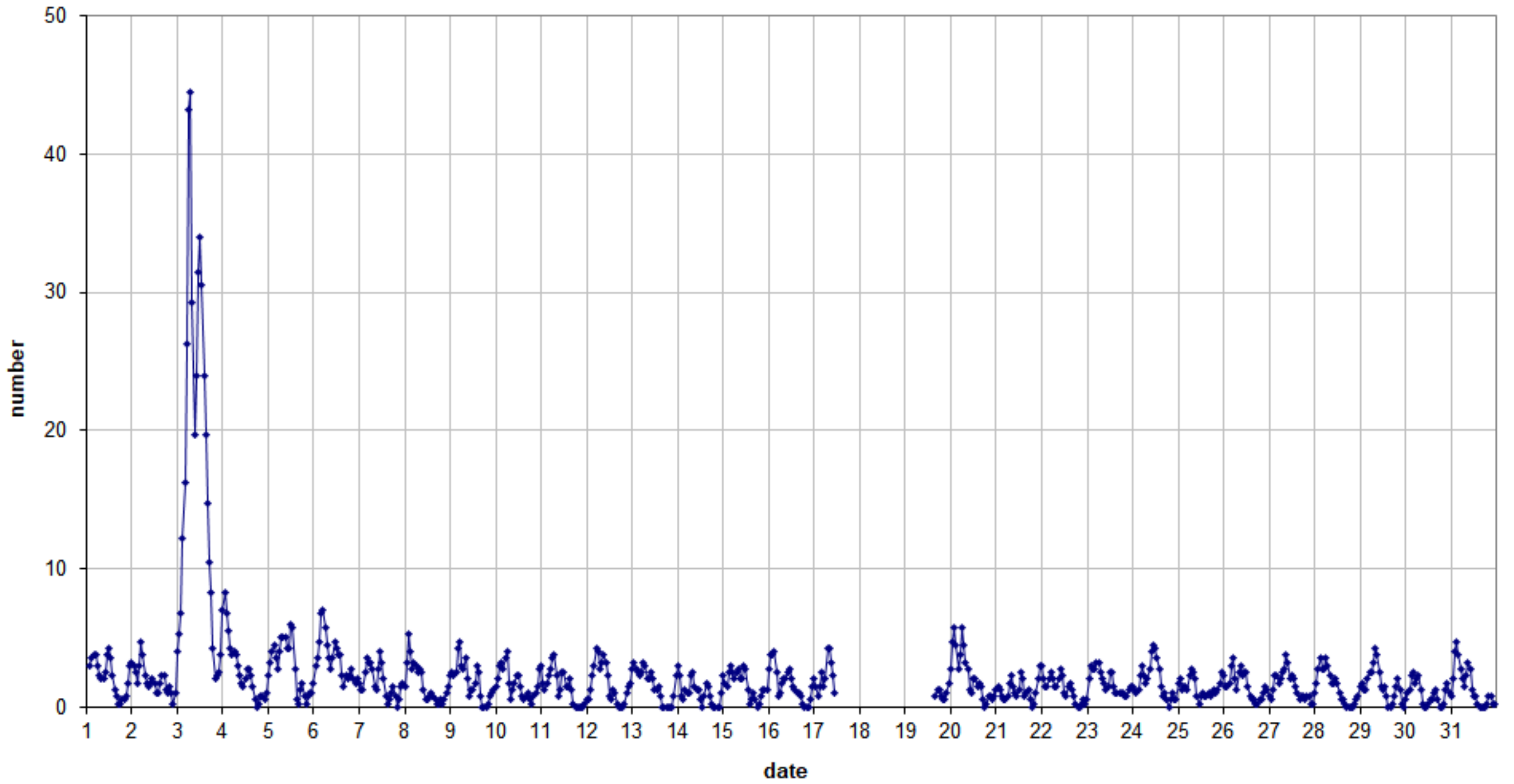
49.99MHz - RadioMeteors January 2025 number of overdense reflections per hour (weighted average) Felix Verbelen (Kampenhout)
