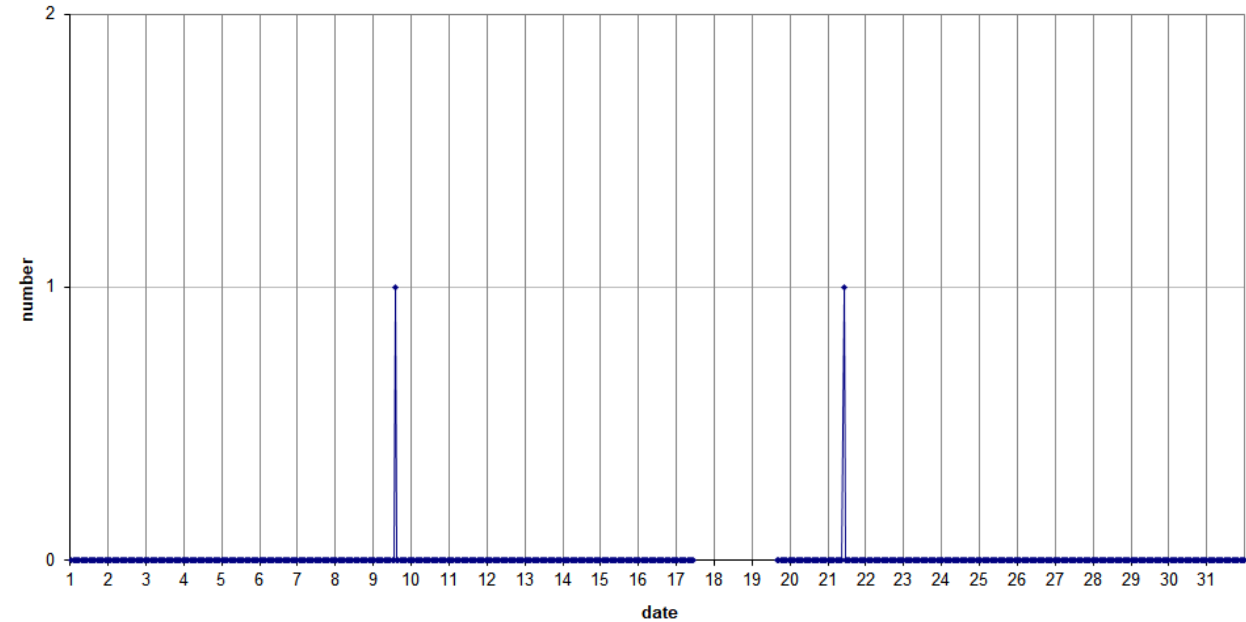
49.99MHz - RadioMeteors January 2025 hourly totals of overdense reflections longer than 1 minute Felix Verbelen (Kampenhout/BE)
