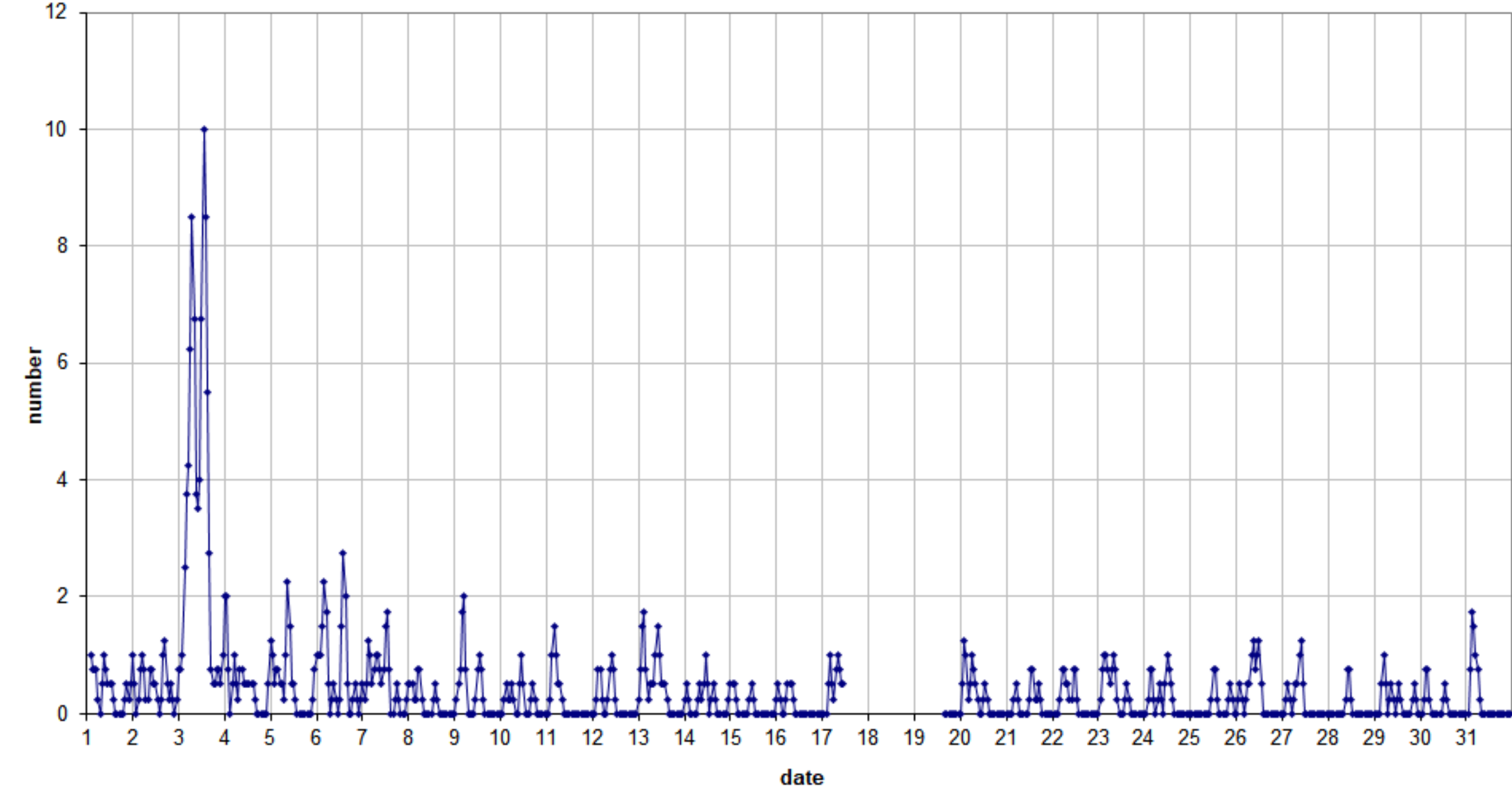
49.99MHz - RadioMeteors January 2025 number of reflections >10 seconds per hour (weighted average) Felix Verbelen (Kampenhout)
