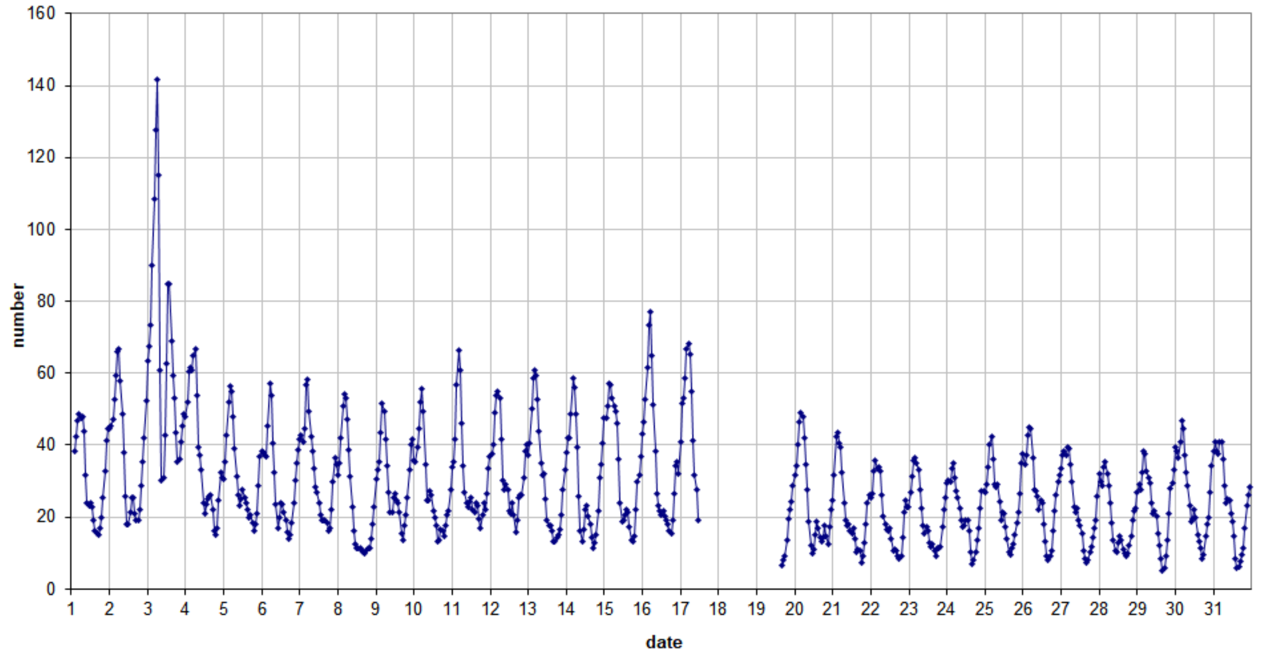
49.99 MHz - RadioMeteors January 2025 number of "all" refections per hour (weighted average) (automatic count_Mettel5_7Hz) Felix Verbelen (Kampenhout)
