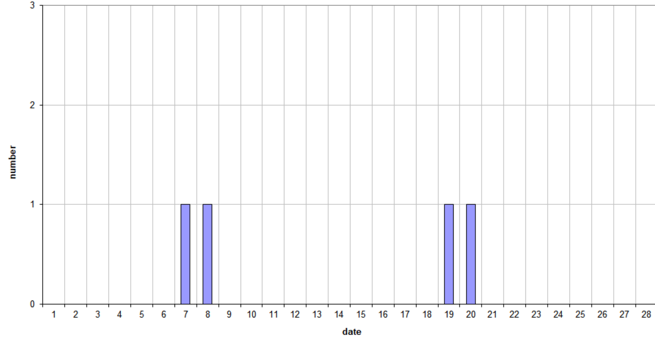
49.99MHz - RadioMeteors February 2025 daily totals of reflections longer than 1 minute Felix Verbelen (Kamphenhout)
