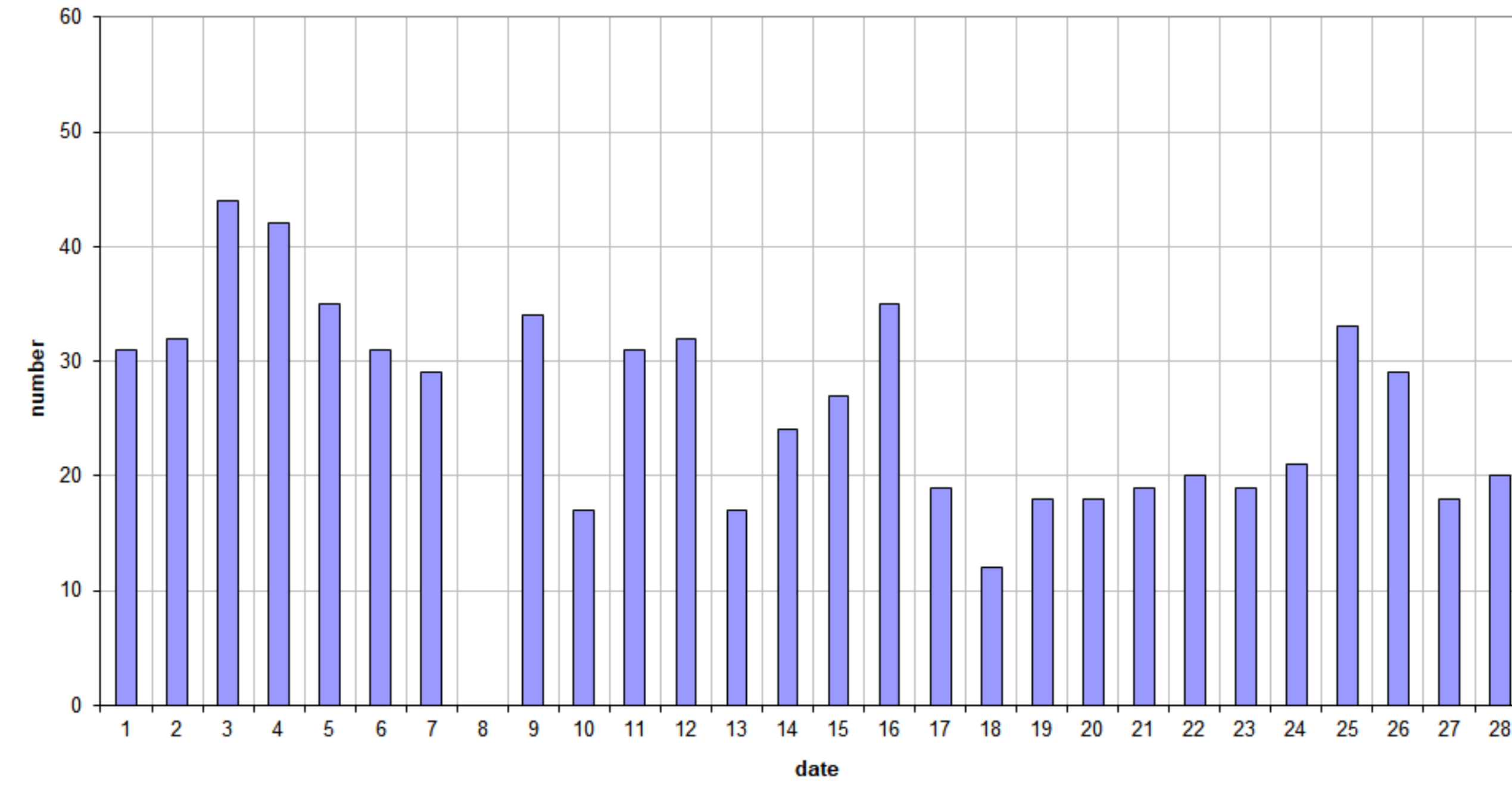
49.99MHz - RadioMeteors February 2025 daily totals of all overdense reflections Felix Verbelen (Kamphenhout)
