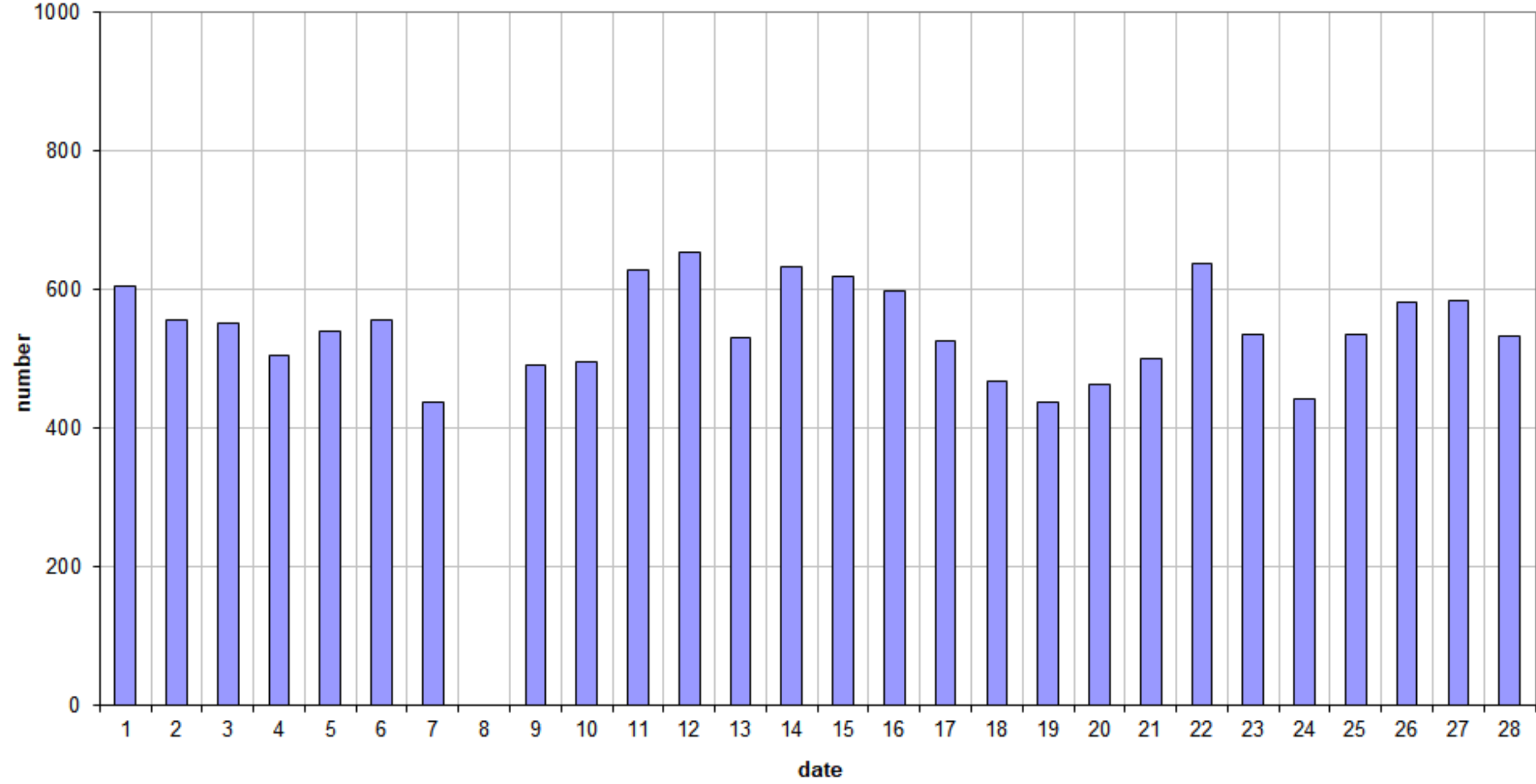
49.99MHz - RadioMeteors February 2025 daily totals of "all" reflections (automatic count_Mettel5_7Hz) Felix Verbelen (Kamphenhout)
