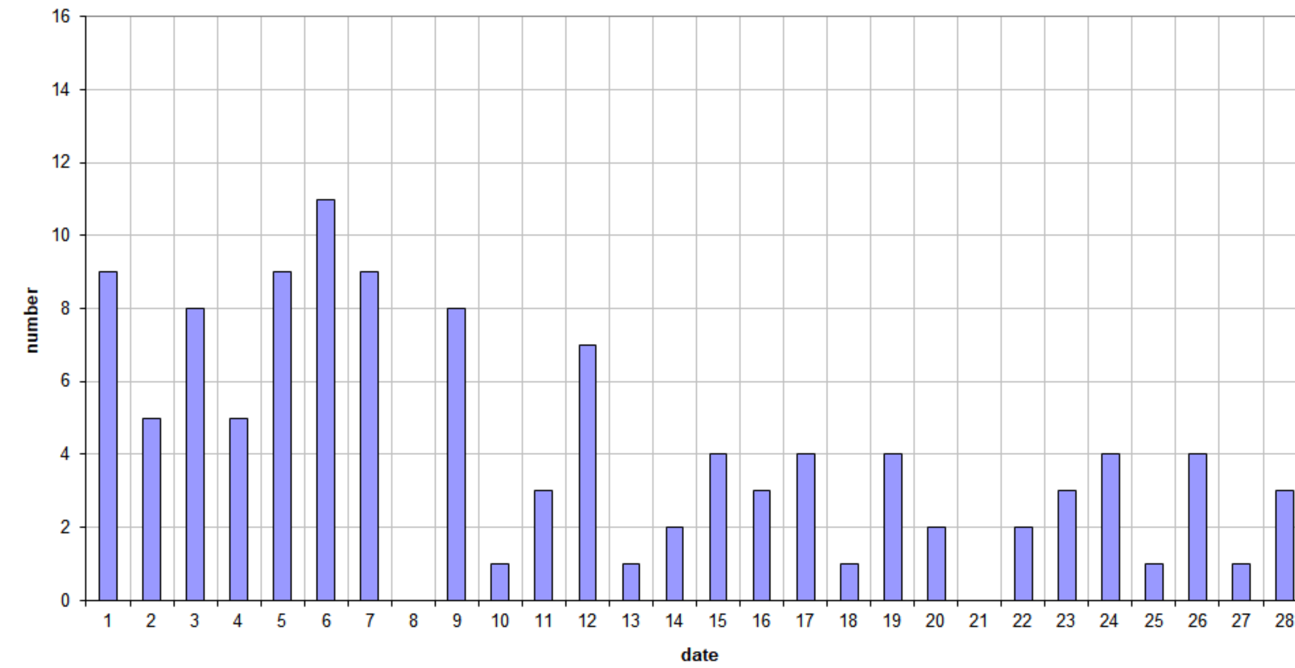
49.99MHz - RadioMeteors February 2025 daily totals of reflections longer than 10 seconds Felix Verbelen (Kamphenhout)
