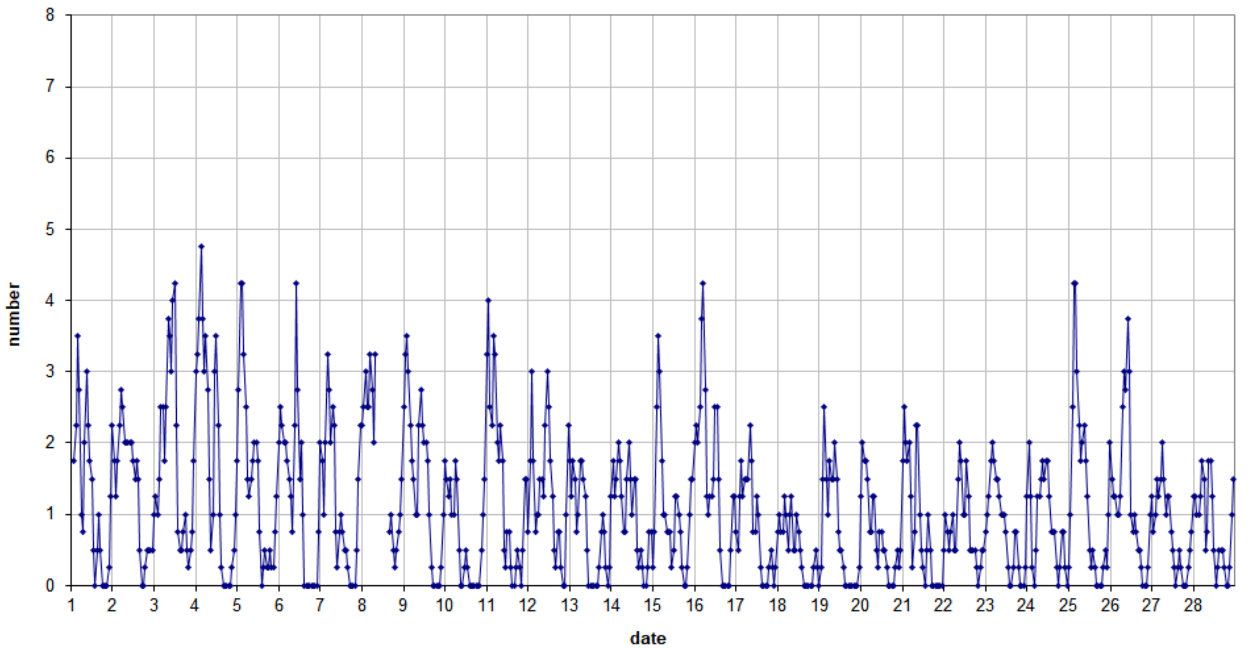
49.99MHz - RadioMeteors February 2025 number of overdense reflections per hour (weighted average) Felix Verbelen (Kampenhout)
