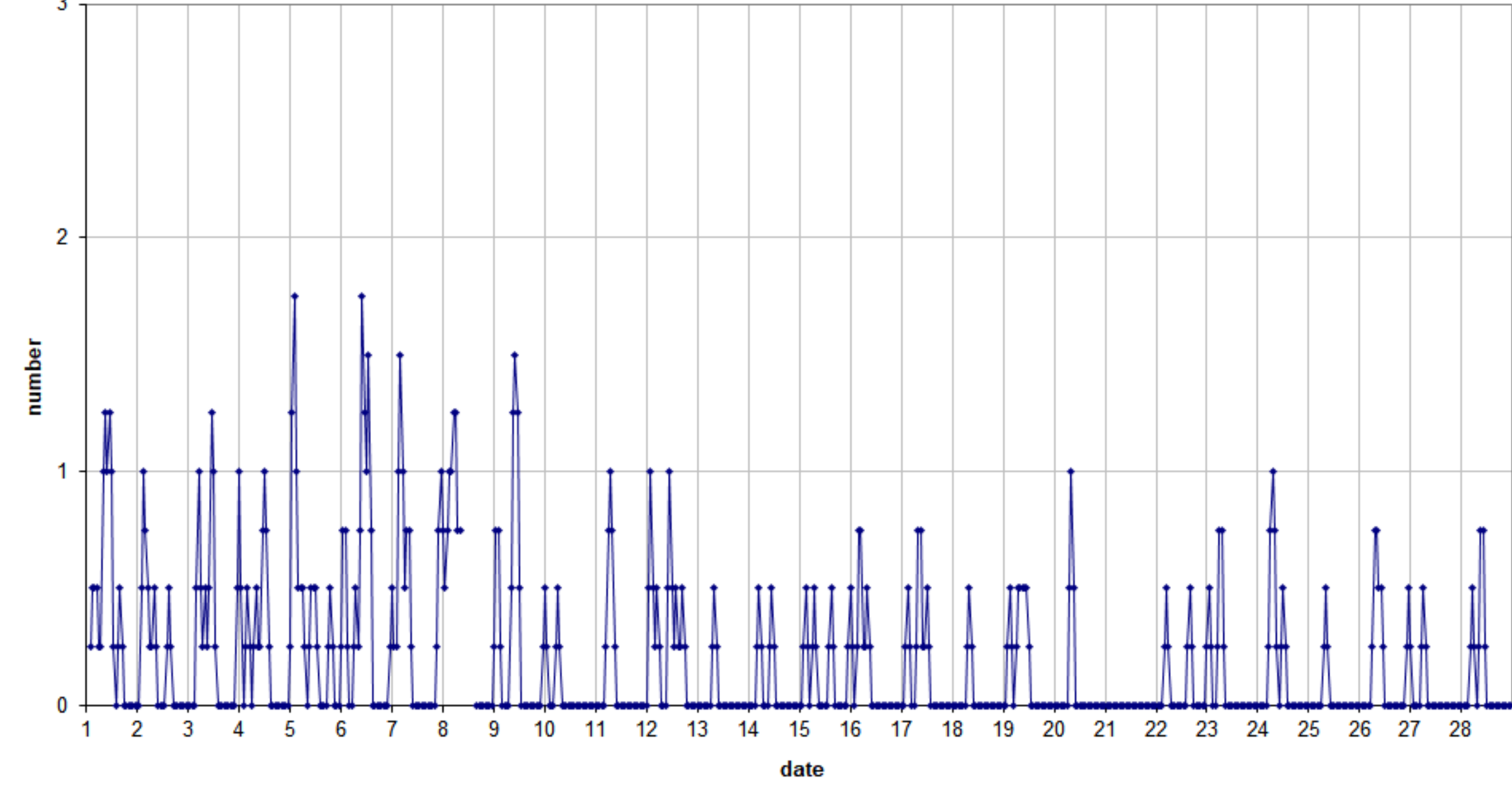
49.99MHz - RadioMeteors February 2025 number of reflections >10 seconds per hour (weighted average) Felix Verbelen (Kampenhout)
