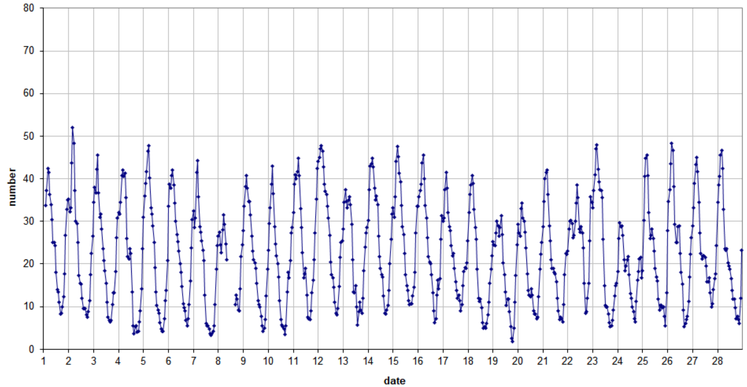
49.99 MHz - RadioMeteors February 2025 number of "all" reflections per hour (weighted average) (automatic count_Mettel5_7Hz) Felix Verbelen (Kampenhout)
