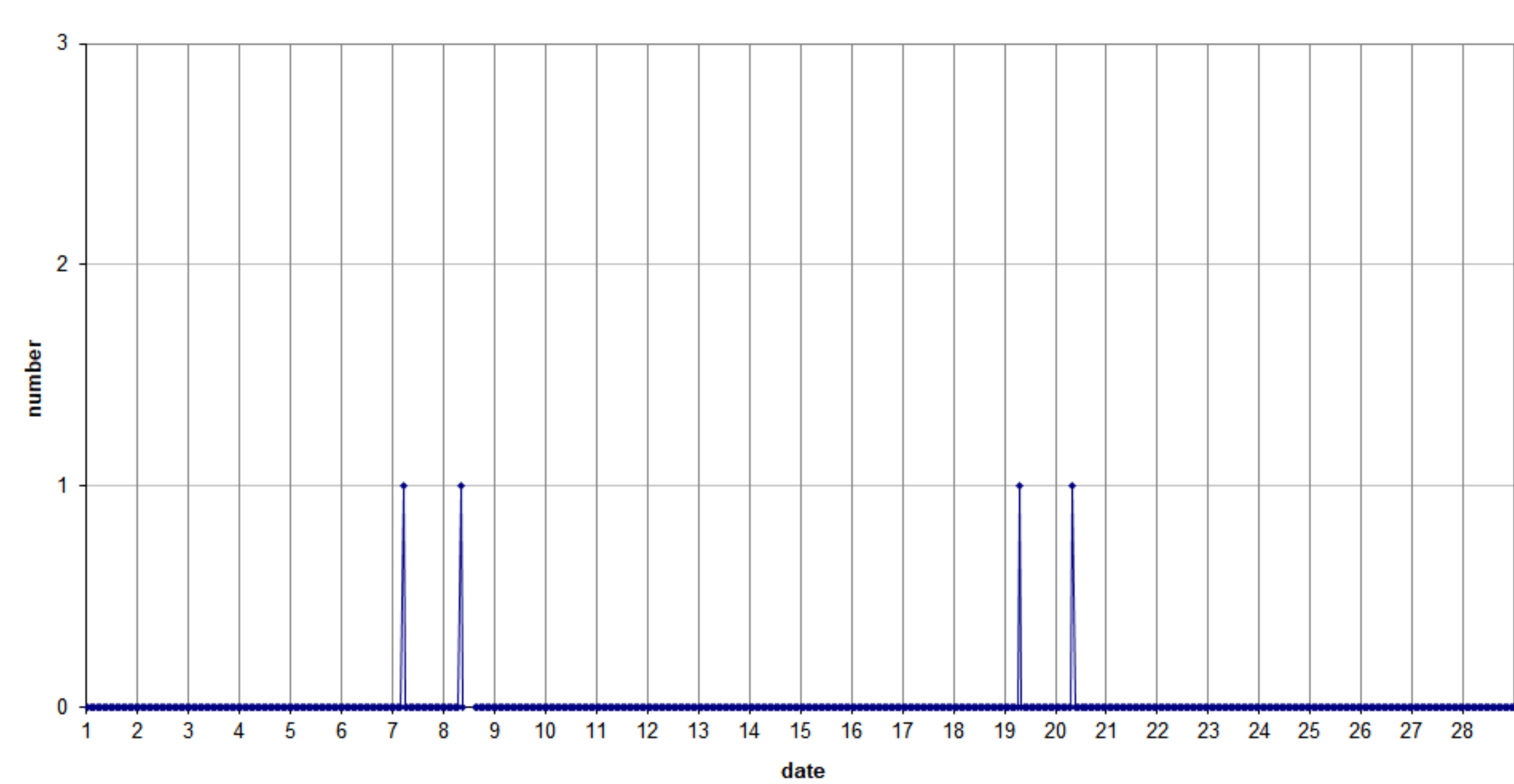
49.99MHz - RadioMeteors February 2025 hourly totals of overdense reflections longer than 1 minute Felix Verbelen (Kampenhout/BE)
