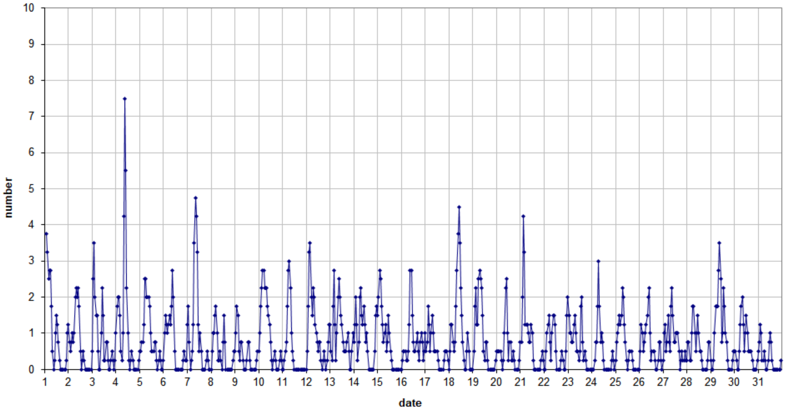
49.99MHz - RadioMeteors March 2025 number of overdense reflections per hour (weighted average) Felix Verbelen (Kamphenhout)
