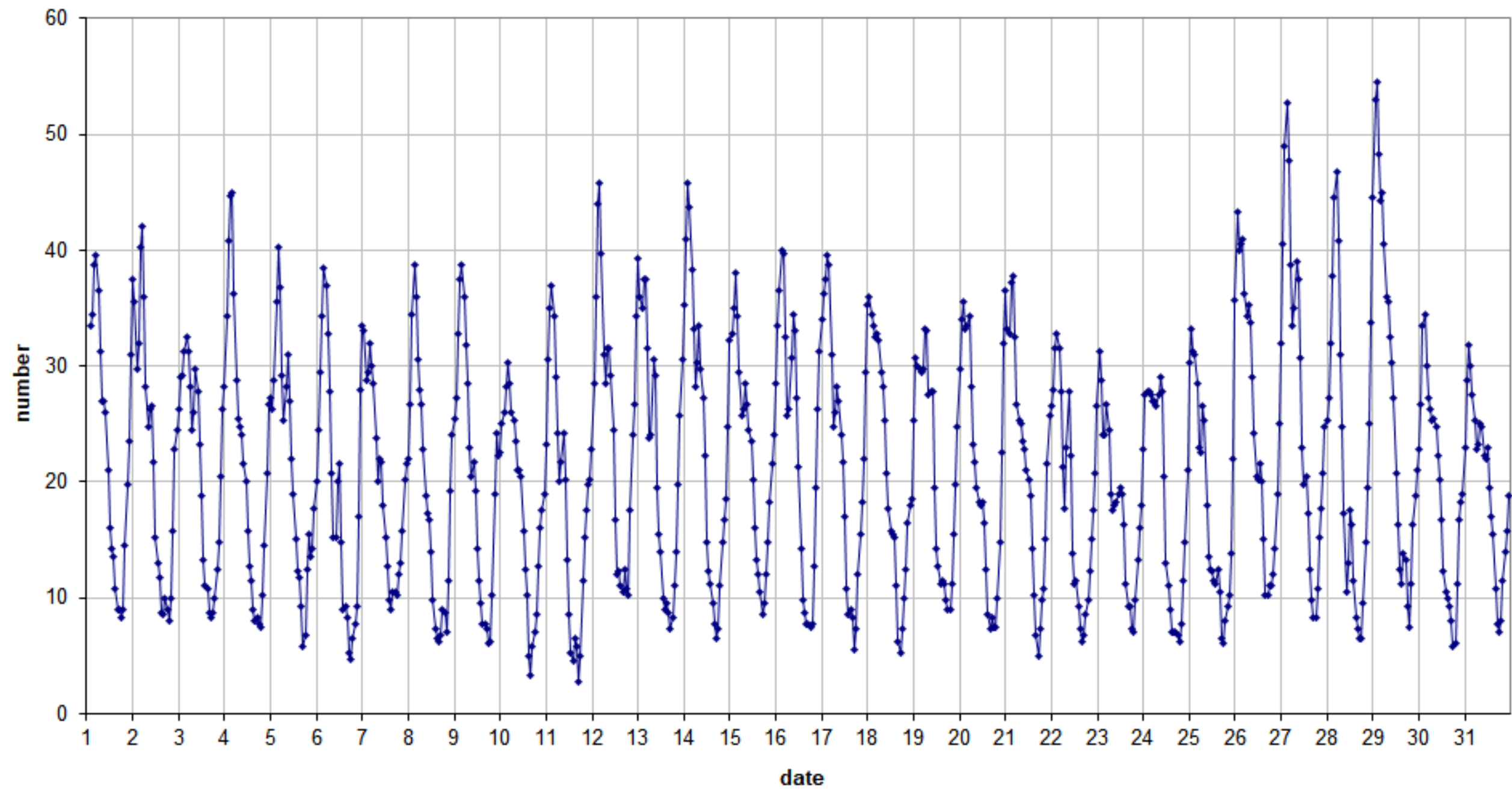
49.99 MHz - RadioMeteors March 2025 number of "all" refections per hour (weighted average) (automatic count_Mettel5_7Hz) Felix Verbelen (Kamphenhout)
