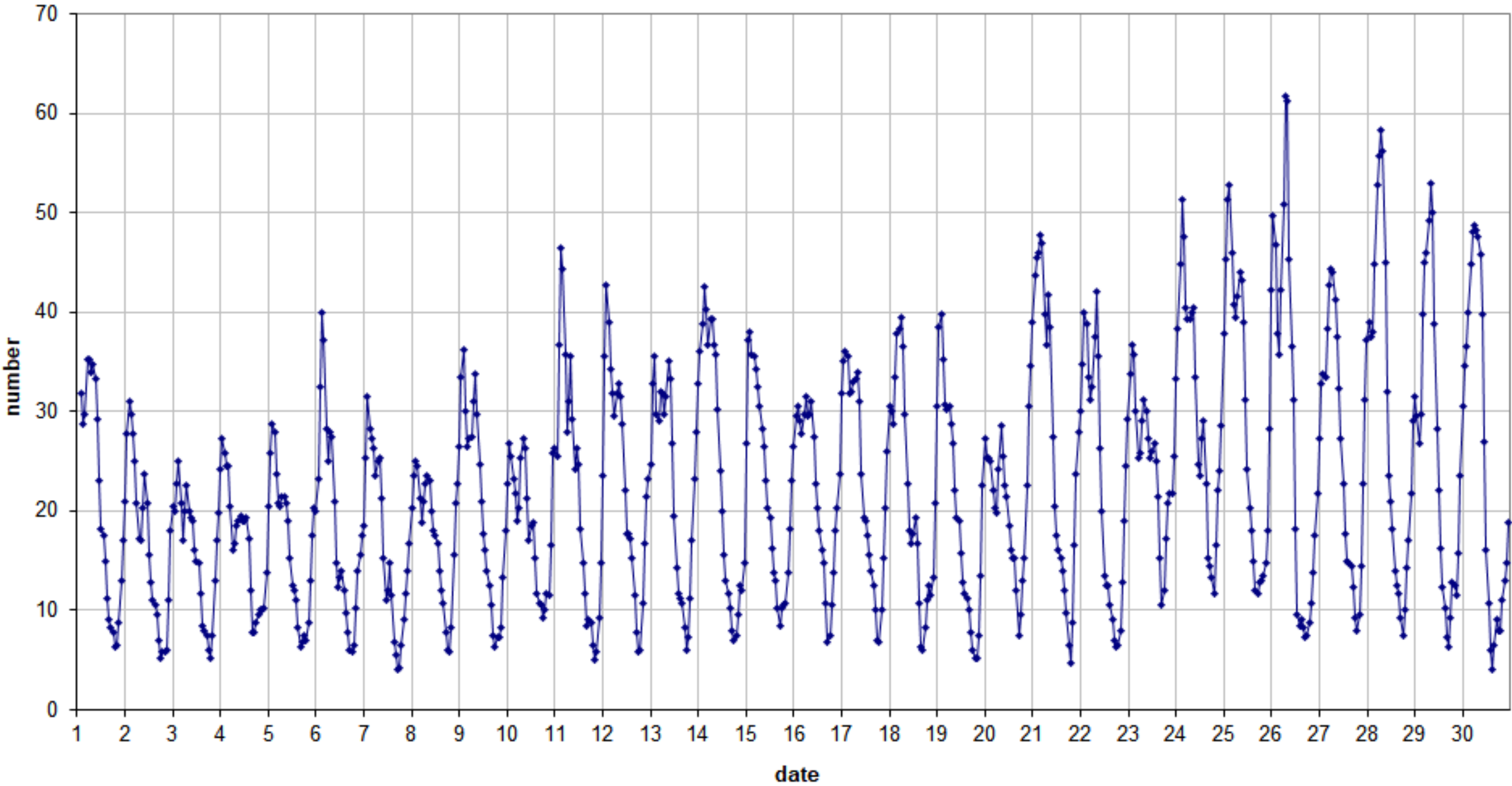
49.99 MHz - RadioMeteors April 2025 number of "all" refections per hour (weighted average) (automatic count_MetteI5_7Hz) Felix Verbelen (Kamphenhout)
