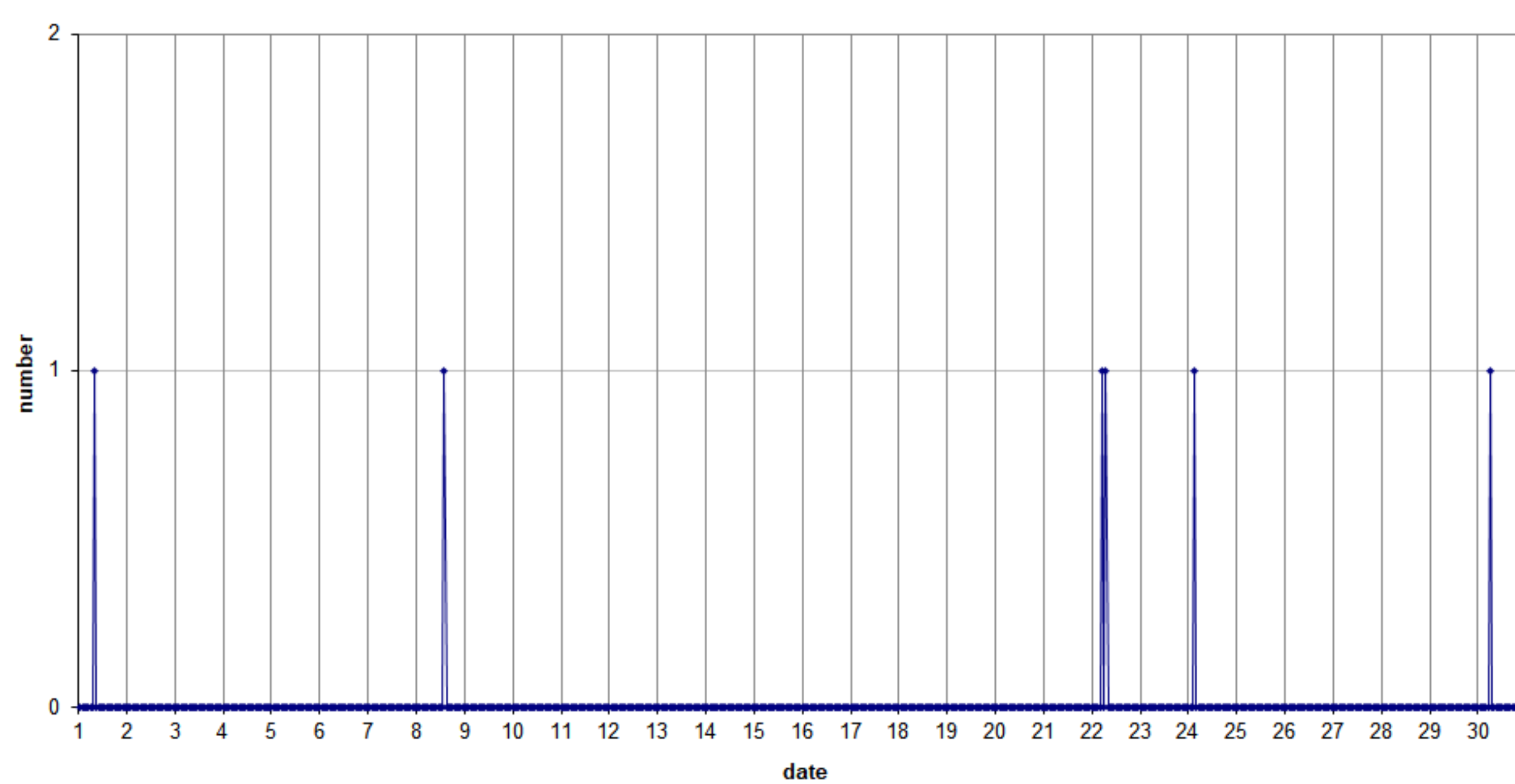
49.99MHz - RadioMeteors April 2025 hourly totals of overdense reflections longer than 1 minute Felix Verbelen (Kamphenhout/BE)
