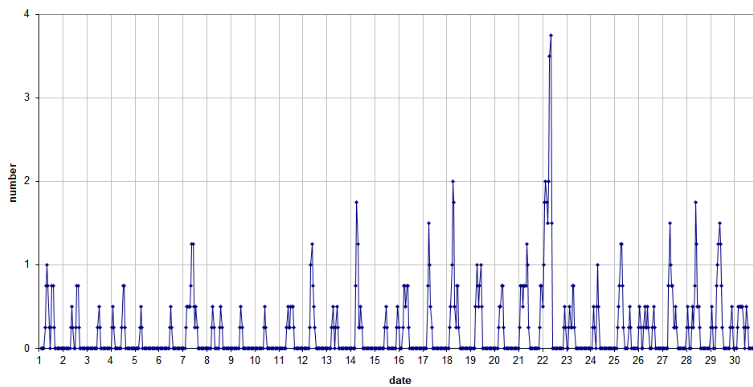
49.99MHz - RadioMeteors April 2025 number of reflections >10 seconds per hour (weighted average) Felix Verbelen (Kamphenhout)
