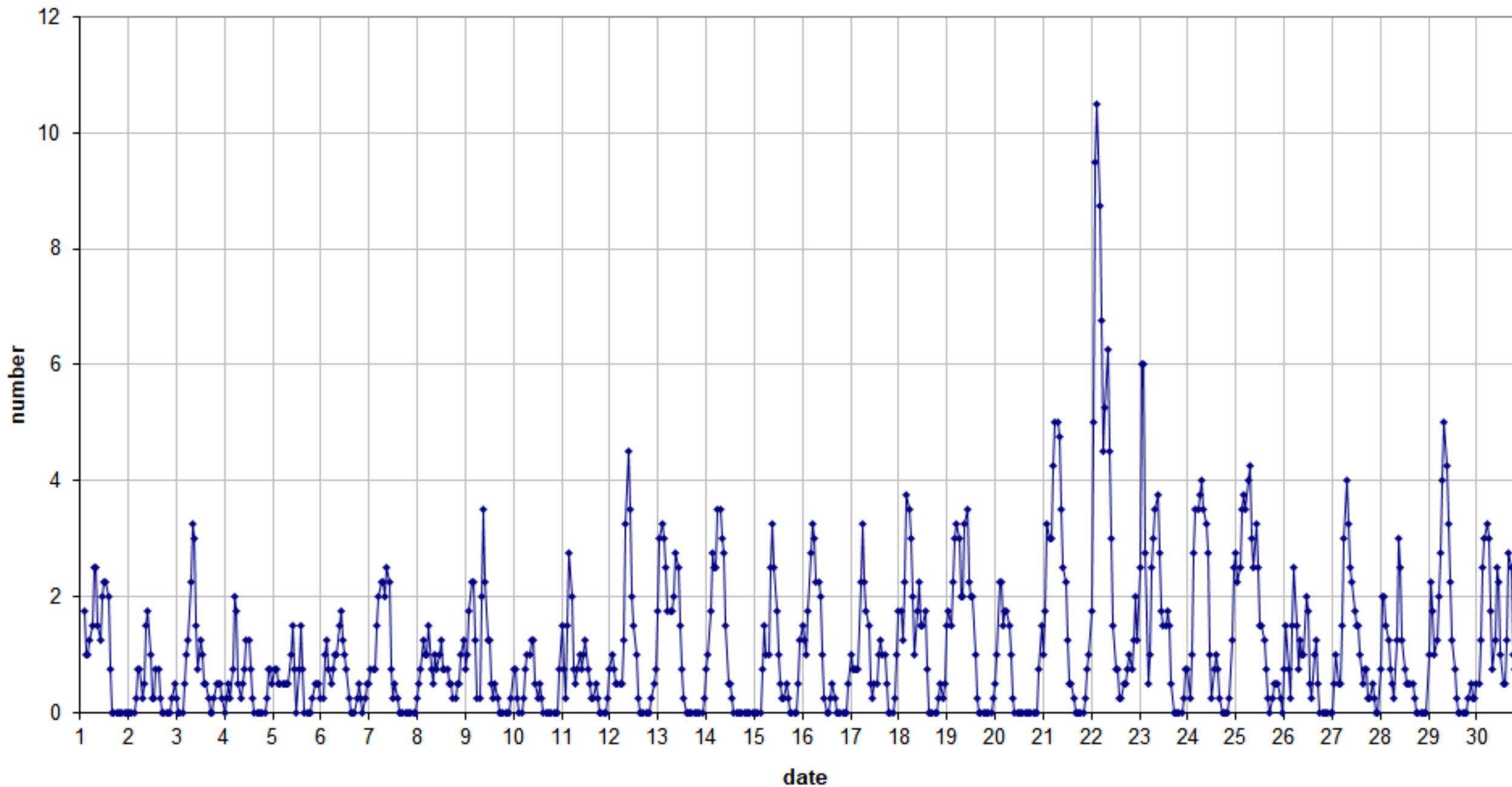
49.99MHz - RadioMeteors April 2025 number of overdense reflections per hour (weighted average) Felix Verbelen (Kamphenhout)
