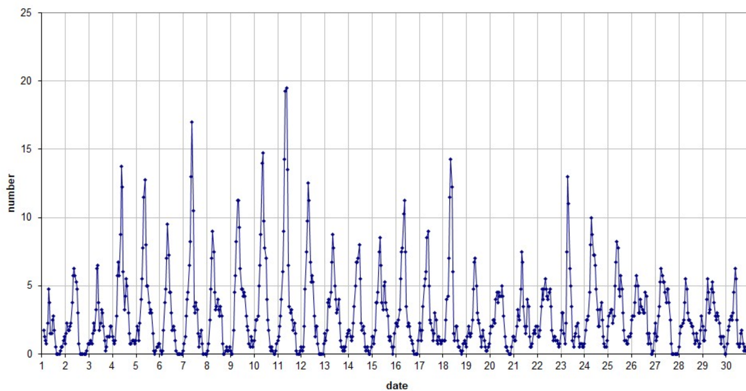
49.99MHz - RadioMeteors June 2025 number of overdense reflections per hour (weighted average) Felix Verbelen (Kampenhout)
