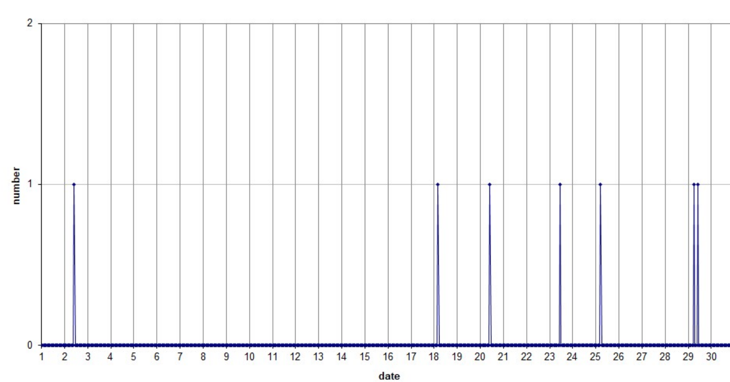
49.99MHz - RadioMeteors June 2025 hourly totals of overdense reflections longer than 1 minute Felix Verbelen (Kampenhout/BE)
