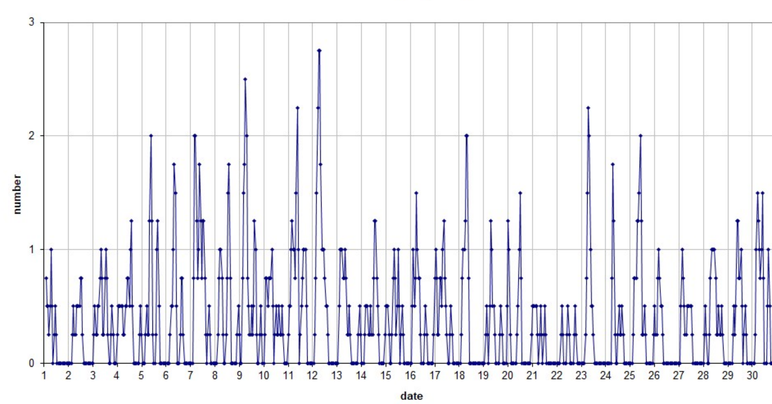
49.99MHz - RadioMeteors June 2025 number of reflections >10 seconds per hour (weighted average) Felix Verbelen (Kampenhout)
