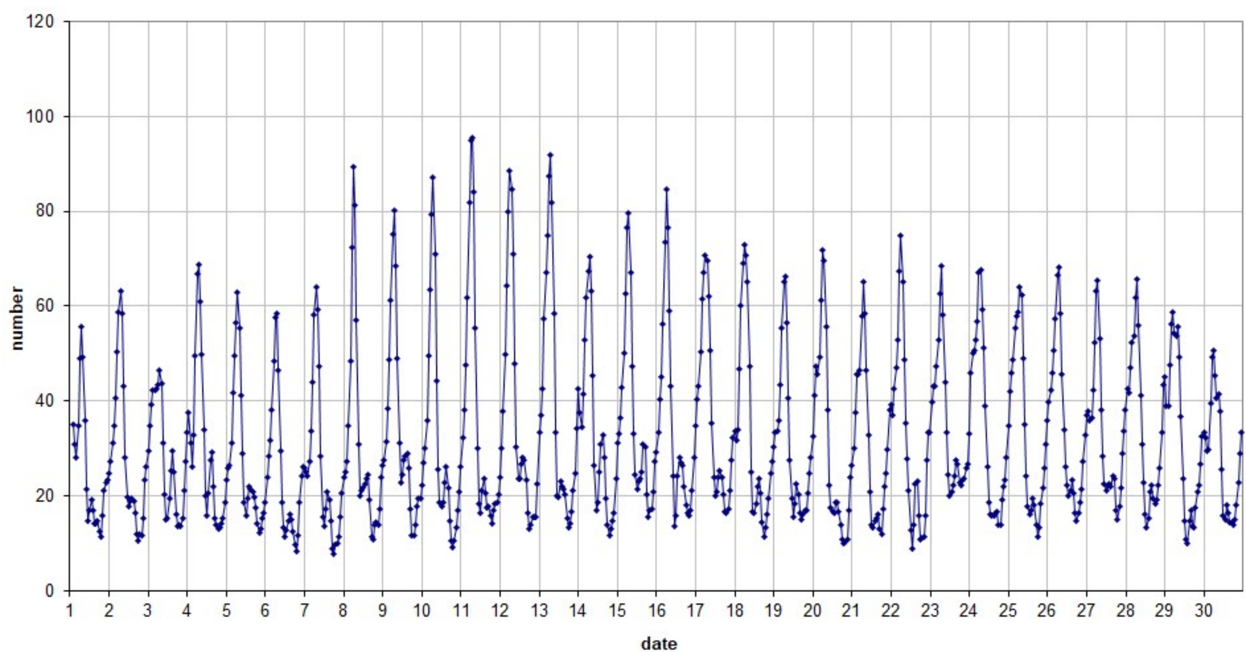
49.99 MHz - RadioMeteors June 2025 number of "all" refections per hour (weighted average) (automatic count_MetteI5_7Hz) Felix Verbelen (Kampenhout)
