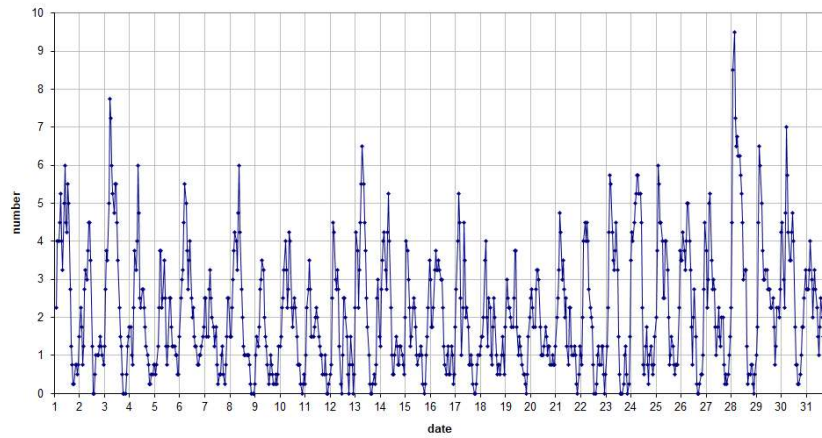
49.99MHz - RadioMeteors July 2025 number of overdense reflections per hour (weighted average) Felix Verbelen (Kamphenhout)
