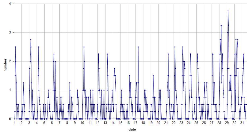
49.99MHz - RadioMeteors July 2025 number of reflections >10 seconds per hour (weighted average) Felix Verbelen (Kamphenhout)
