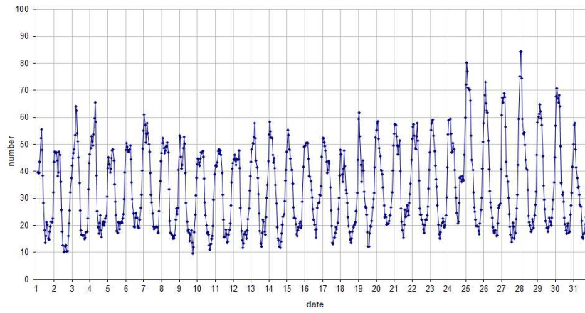
49.99 MHz - RadioMeteors July 2025 number of "all" reflections per hour (weighted average) (automatic count_Mette15_7Hz) Felix Verbelen (Kamphenhout)
