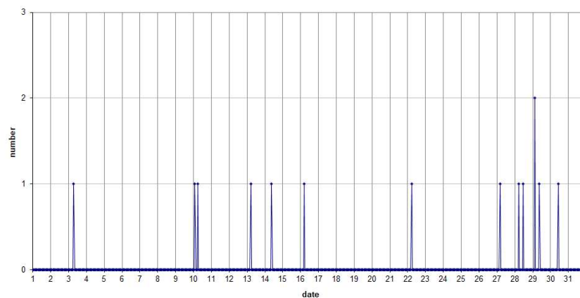
49.99MHz - RadioMeteors July 2025 hourly totals of overdense reflections longer than 1 minute Felix Verbelen (Kamphenhout/BE)
