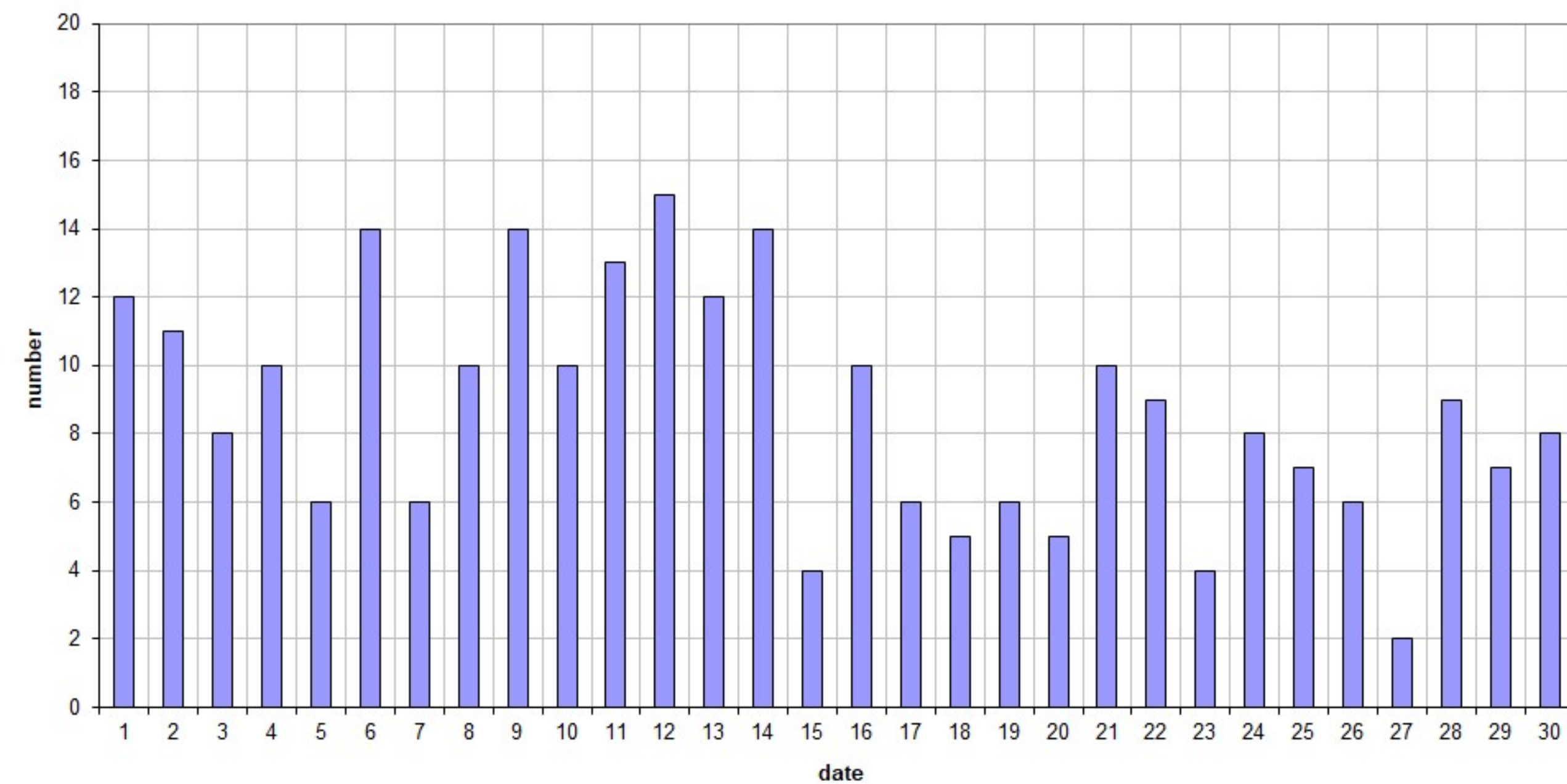
49.99MHz - RadioMeteors September 2025 daily totals of reflections longer than 10 seconds Felix Verbelen (Kamphenhout)
