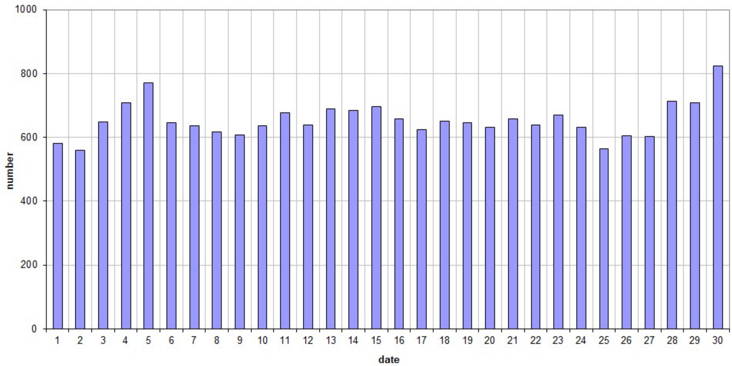
49.99MHz - RadioMeteors September 2025 daily totals of "all" reflections (automatic count_Mettel5_7Hz) Felix Verbelen (Kamphenhout)
