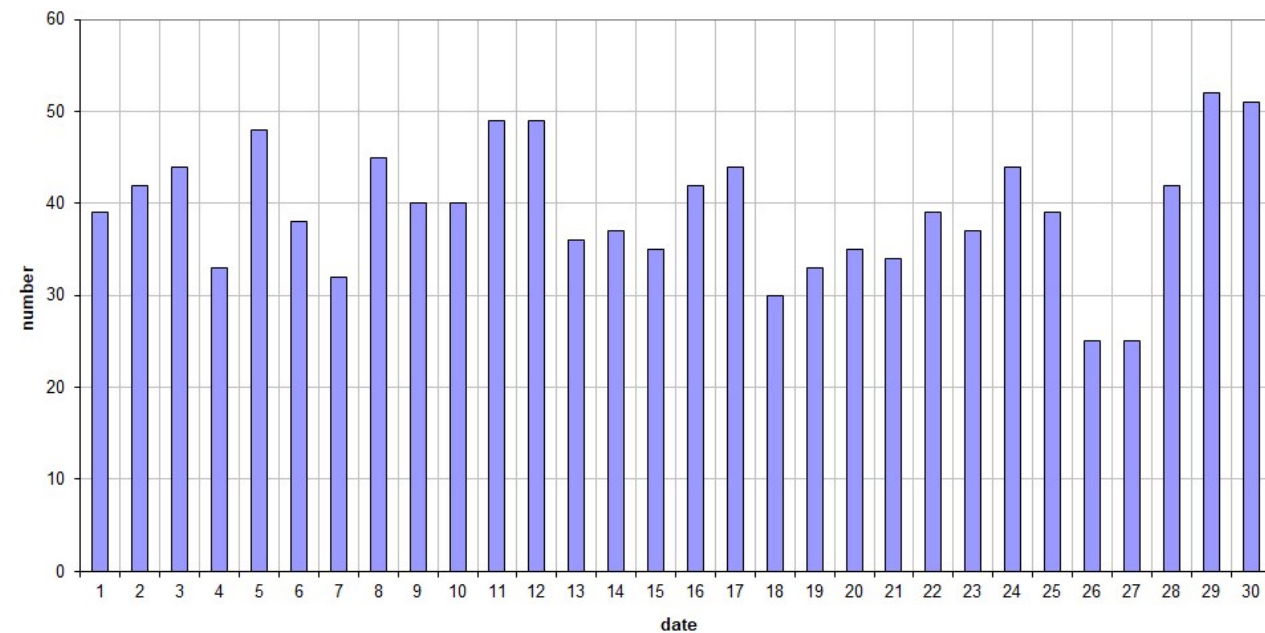
49.99MHz - RadioMeteors September 2025 daily totals of all overdense reflections Felix Verbelen (Kamphenhout)
