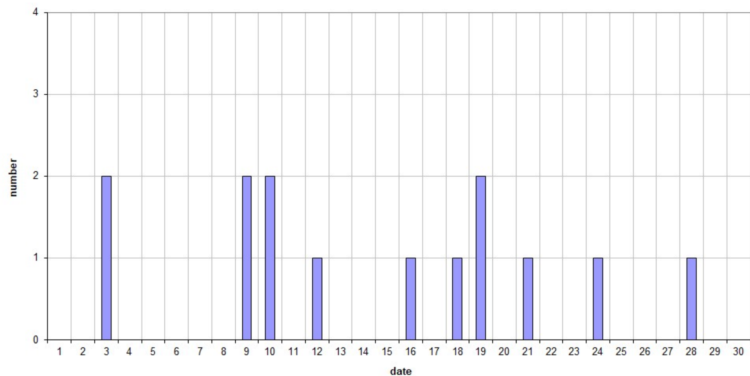
49.99MHz - RadioMeteors September 2025 daily totals of reflections longer than 1 minute Felix Verbelen (Kamphenhout)
