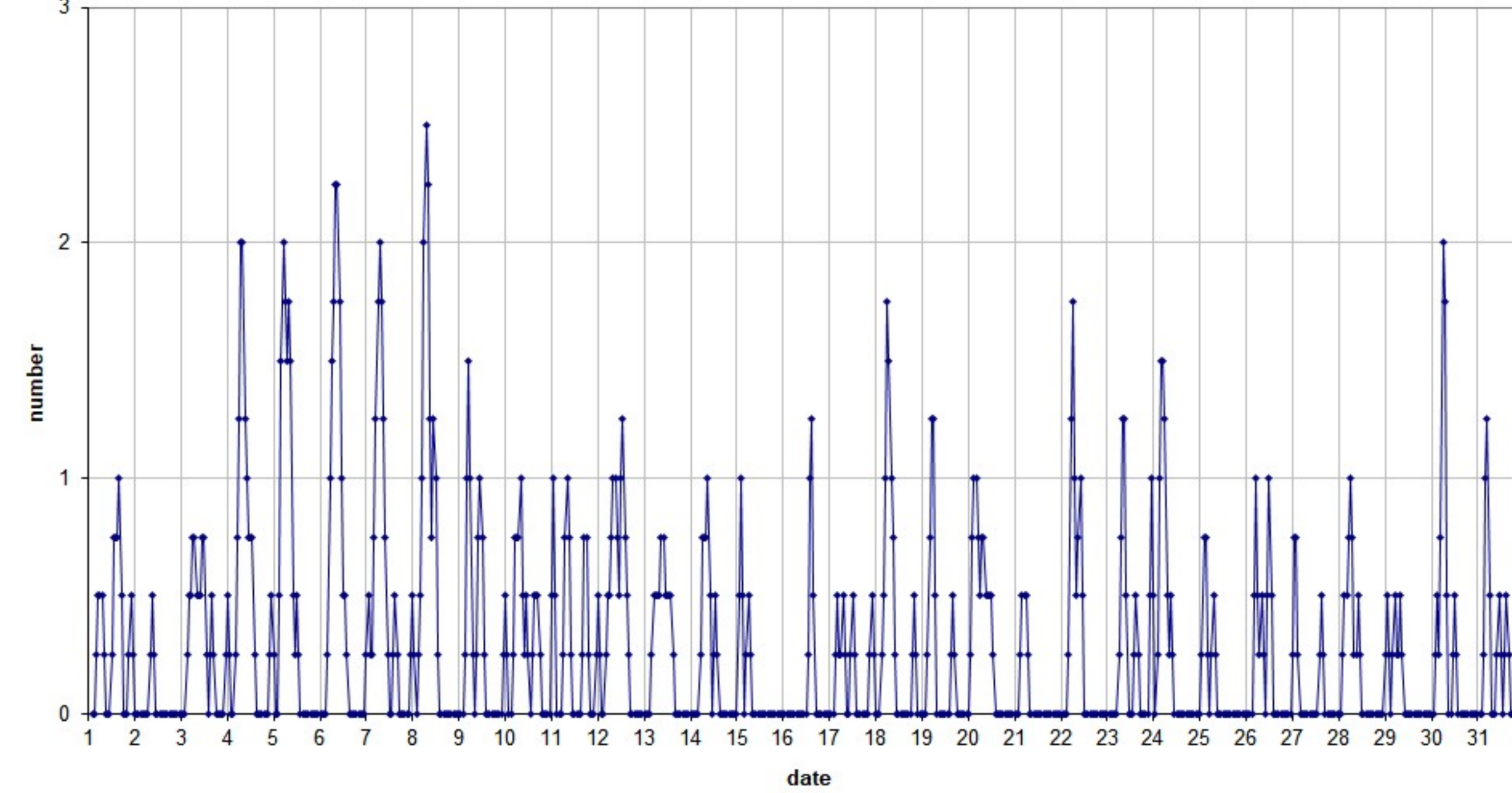
49.99MHz - RadioMeteors May 2026 number of reflections >10 seconds per hour (weighted average) Felix Verbelen (Kamphenhout)
