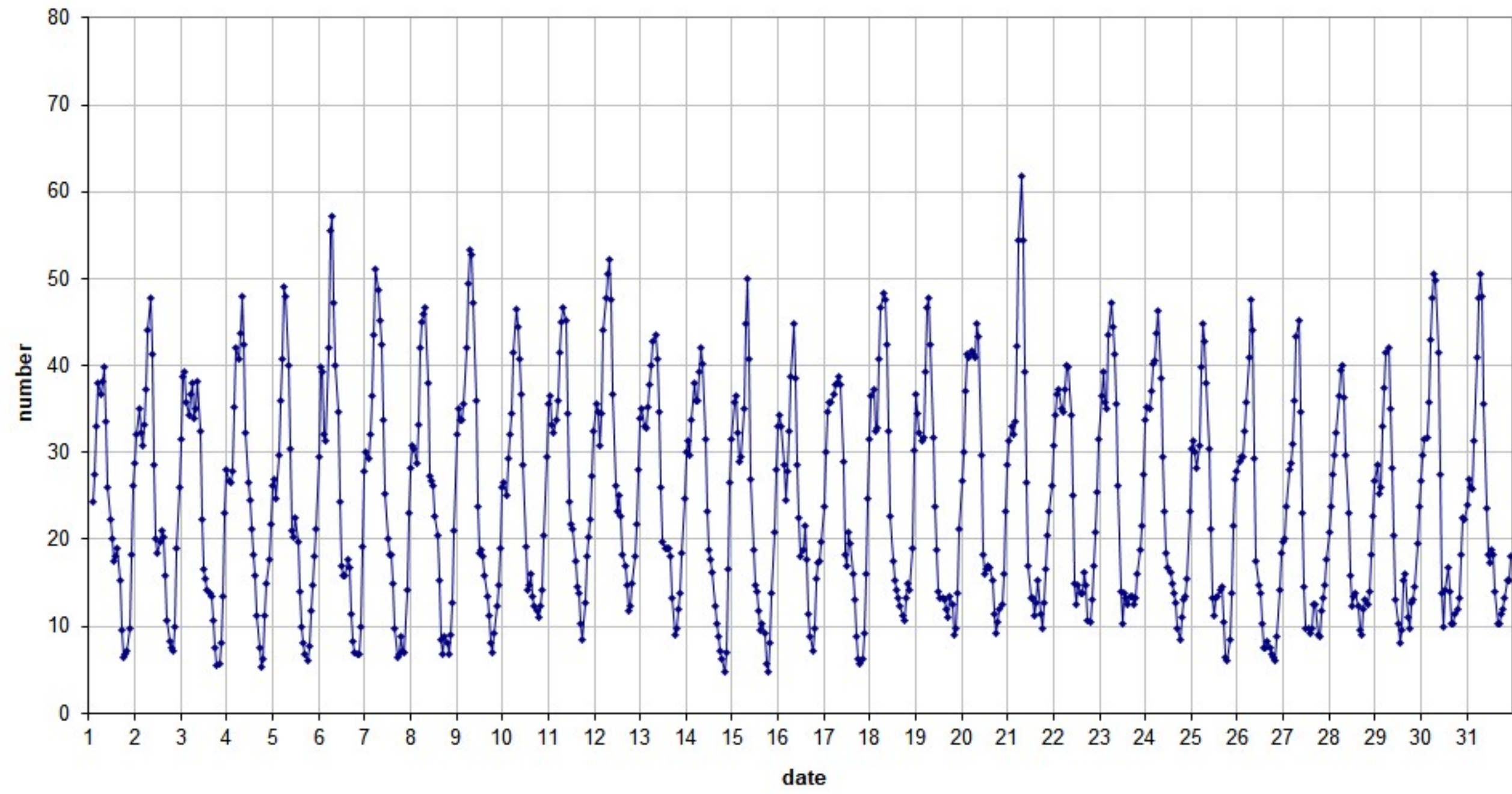
49.99 MHz - RadioMeteors May 2026 number of "all" refections per hour (weighted average) (automatic count_MetteI5_7Hz) Felix Verbelen (Kamphenhout)
