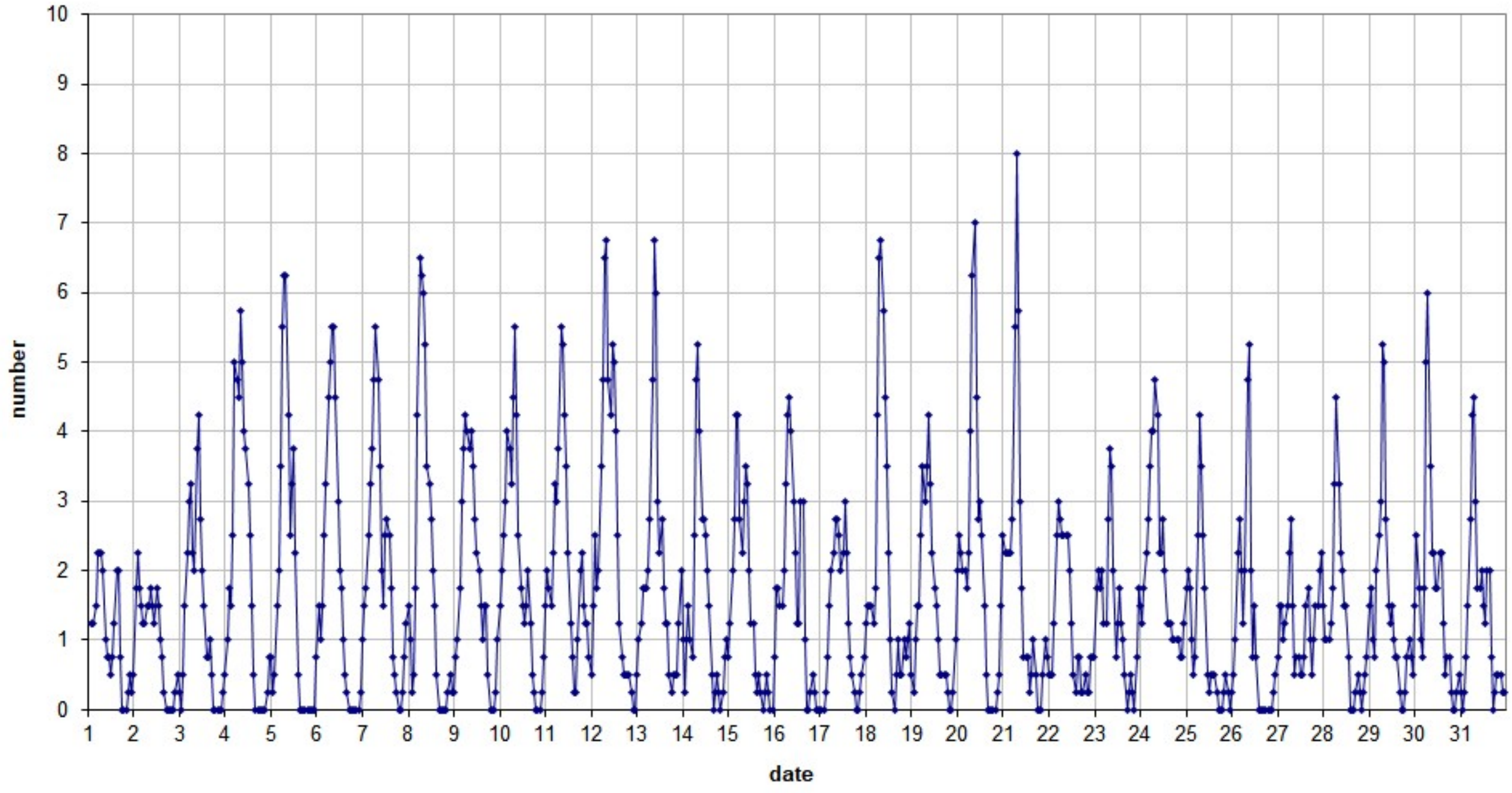
49.99MHz - RadioMeteors May 2026 number of overdense reflections per hour (weighted average) Felix Verbelen (Kamphenhout)
