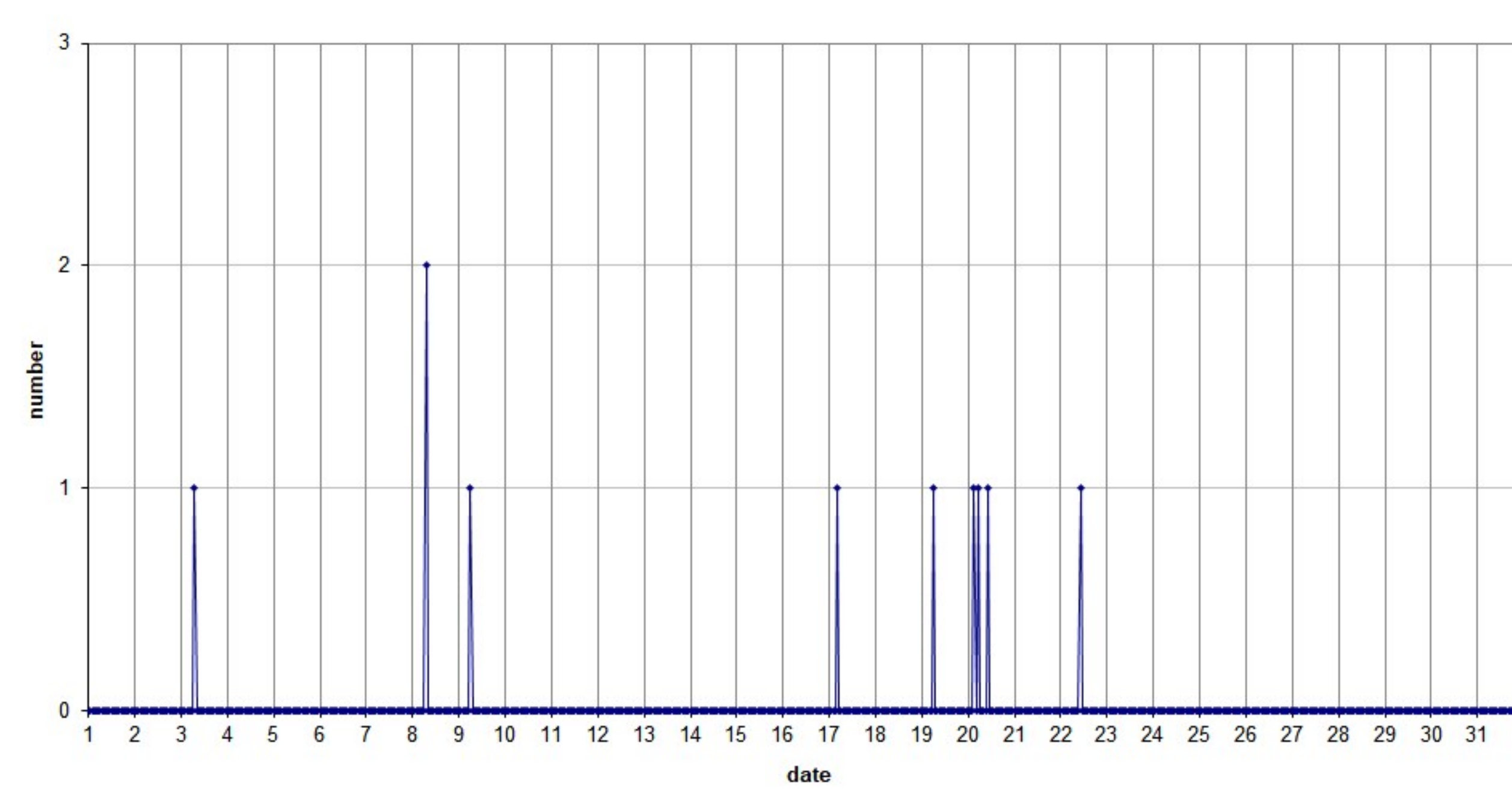
49.99MHz - RadioMeteors May 2026 hourly totals of overdense reflections longer than 1 minute Felix Verbelen (Kamphenhout/BE)
