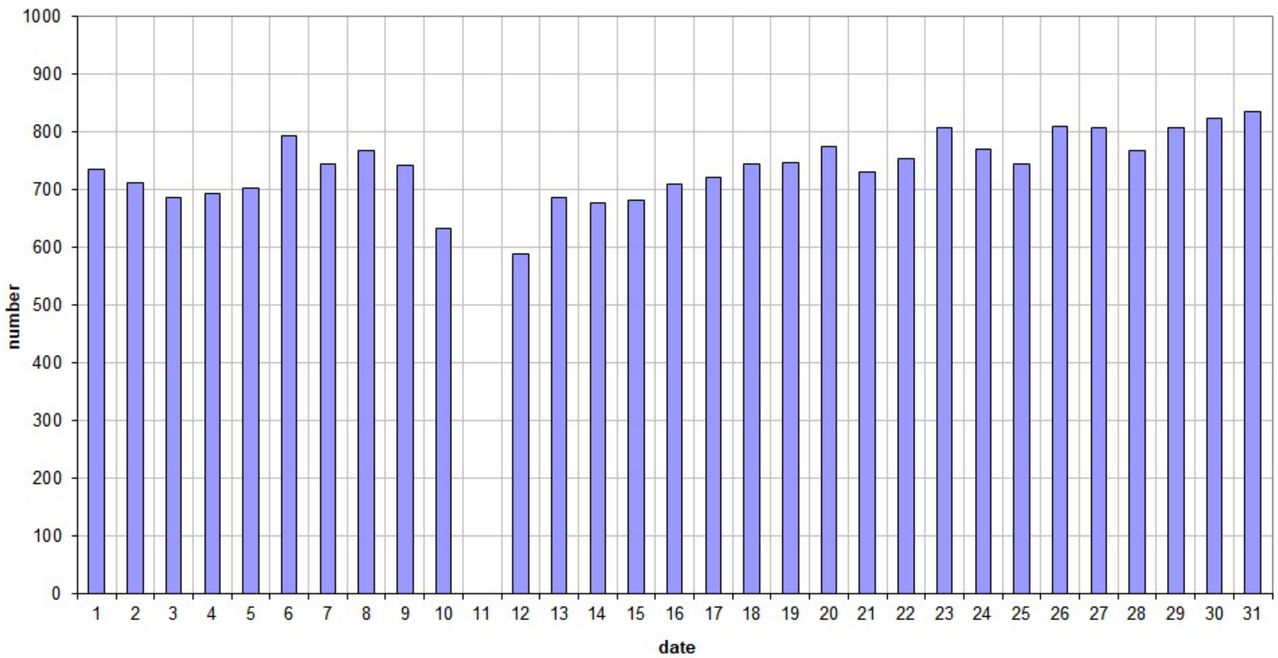
49.99MHz - RadioMeteors July 2026 daily totals of "all" reflections (automatic count_MetteI5_7Hz) Felix Verbelen (Kampenhout)
