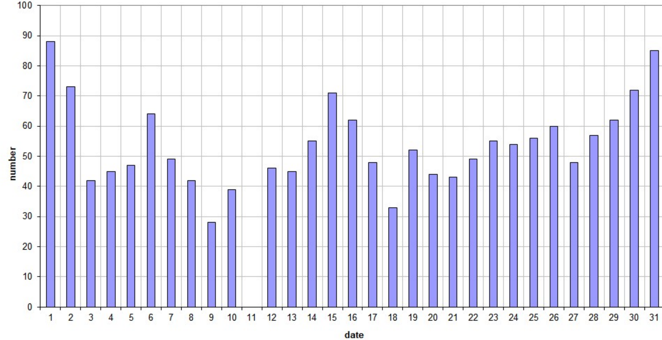
49.99MHz - RadioMeteors July 2026 daily totals of all overdense reflections Felix Verbelen (Kampenhout)
