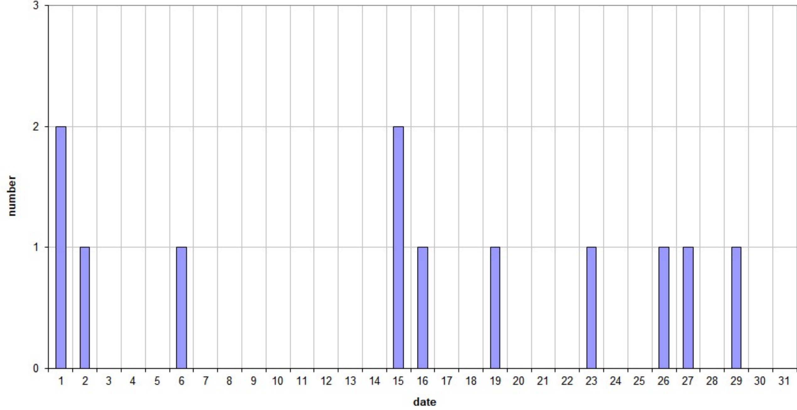
49.99MHz - RadioMeteors July 2026 daily totals of reflections longer than 1 minute Felix Verbelen (Kampenhout)
