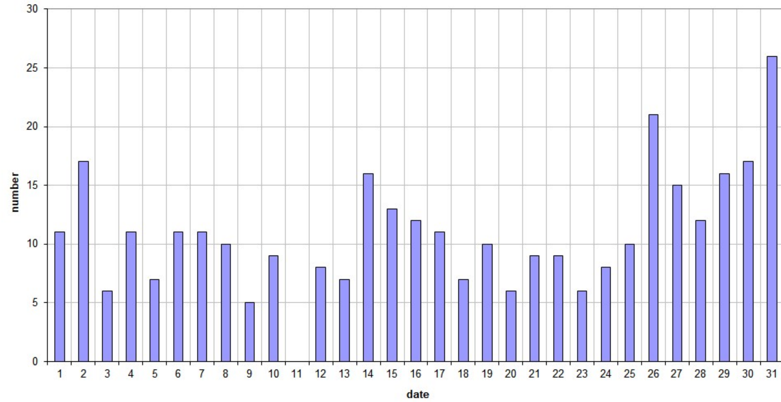
49.99MHz - RadioMeteors July 2026 daily totals of reflections longer than 10 seconds Felix Verbelen (Kampenhout)
