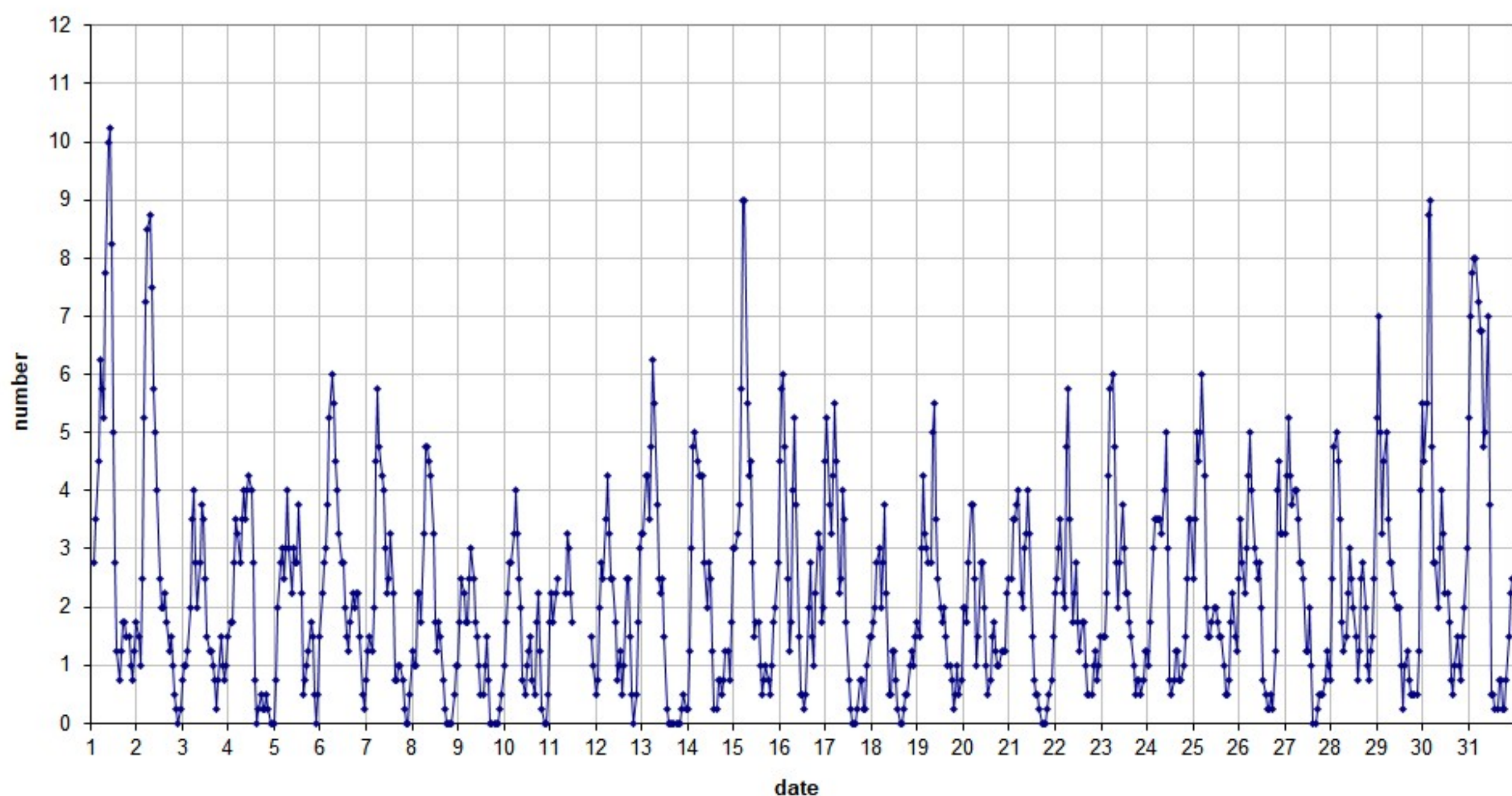
49.99MHz - RadioMeteors July 2026 number of overdense reflections per hour (weighted average) Felix Verbelen (Kampenhout)
